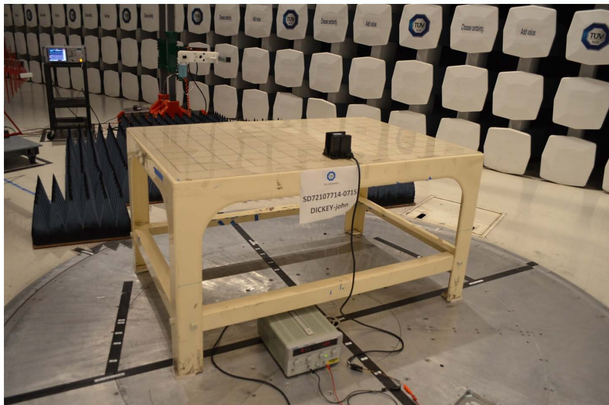
18 GHz to 26 GHz (Back)
