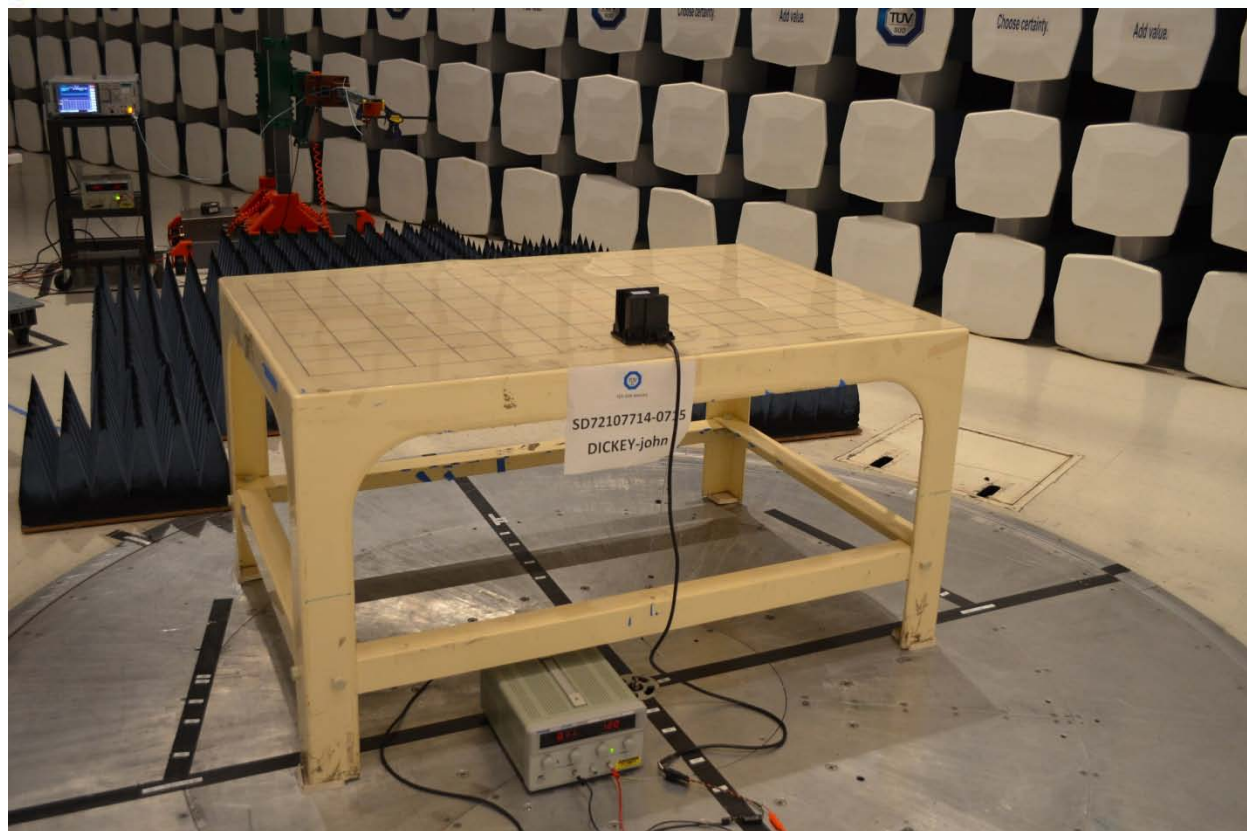
26 GHz to 40 GHz (Back)
