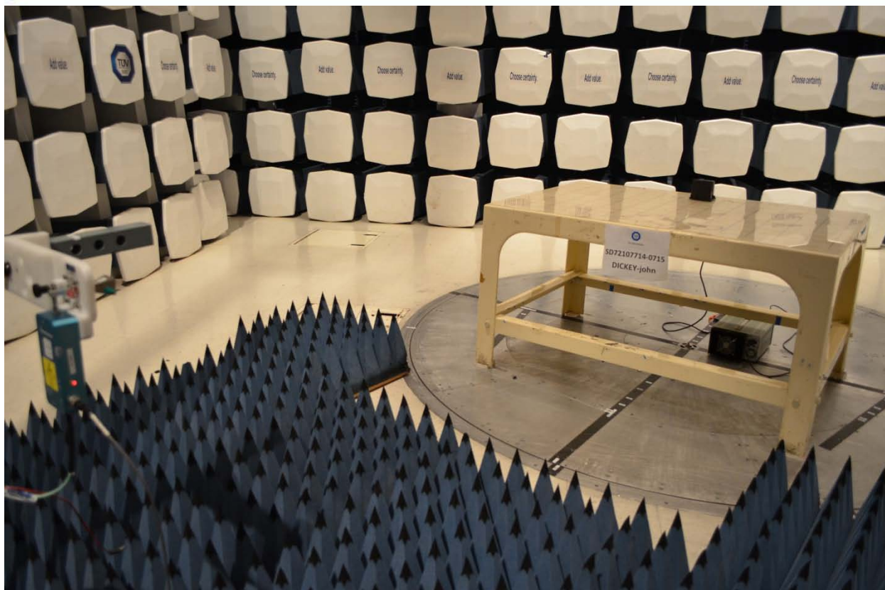
18 GHz to 26 GHz (Front)
