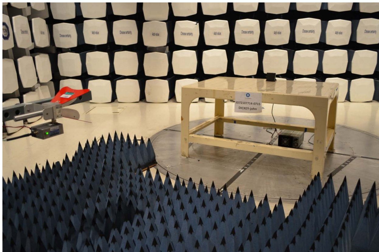
1 GHz to 18 GHz (Front)
