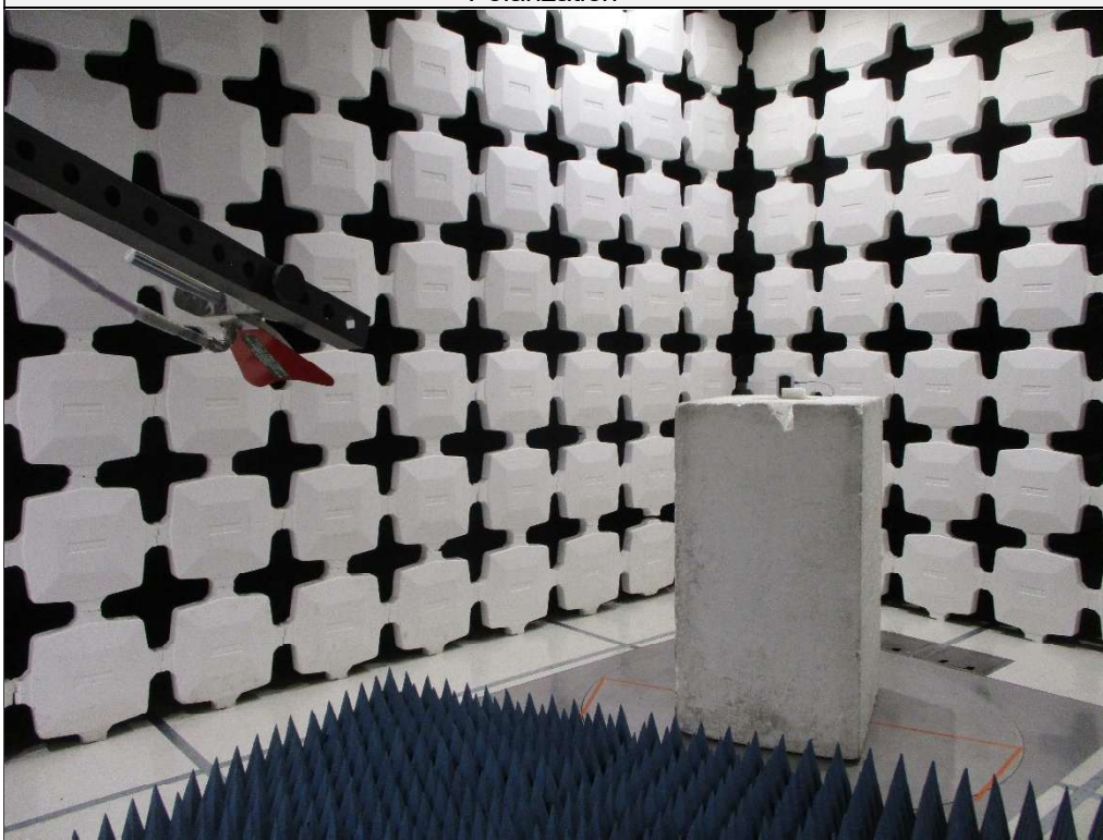
Test Setup for Radiated Spurious Emissions: 1GHz to 4.5GHz, Vertical Polarization
