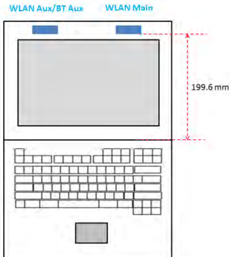
Antenna location (laptop mode)
