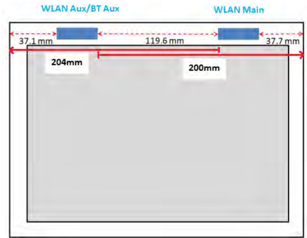
Antenna location (tablet mode, front view)
