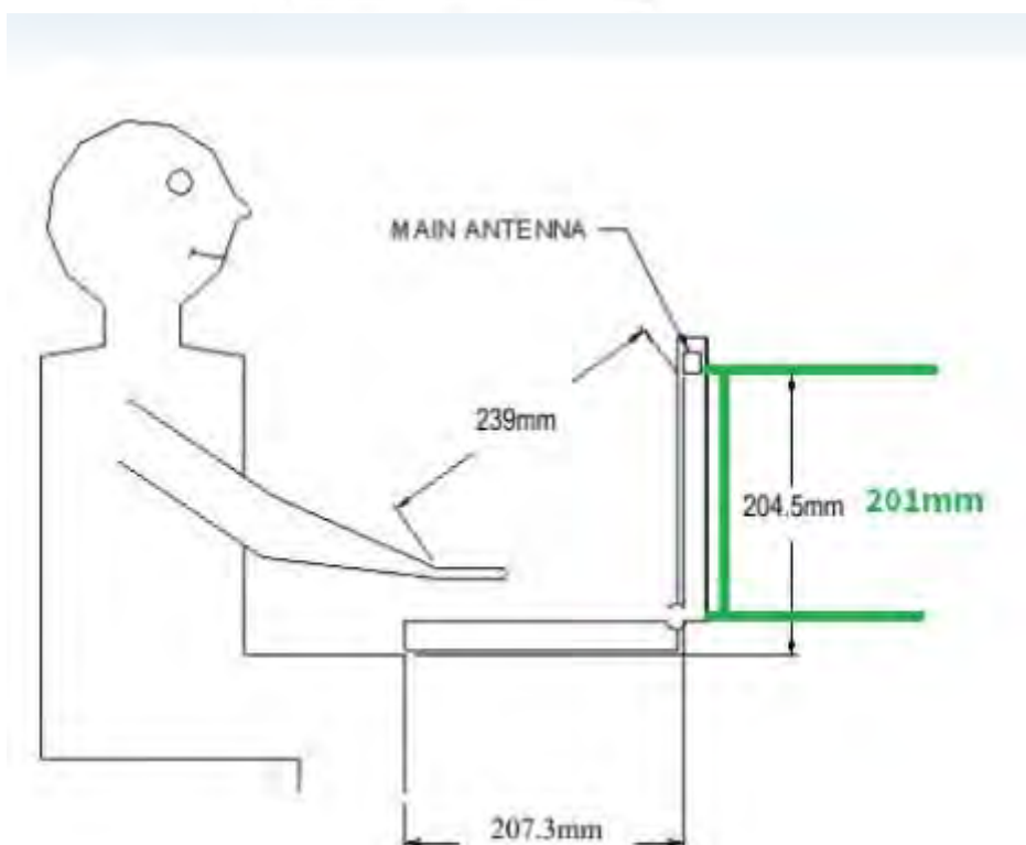
Antenna location (laptop mode)
