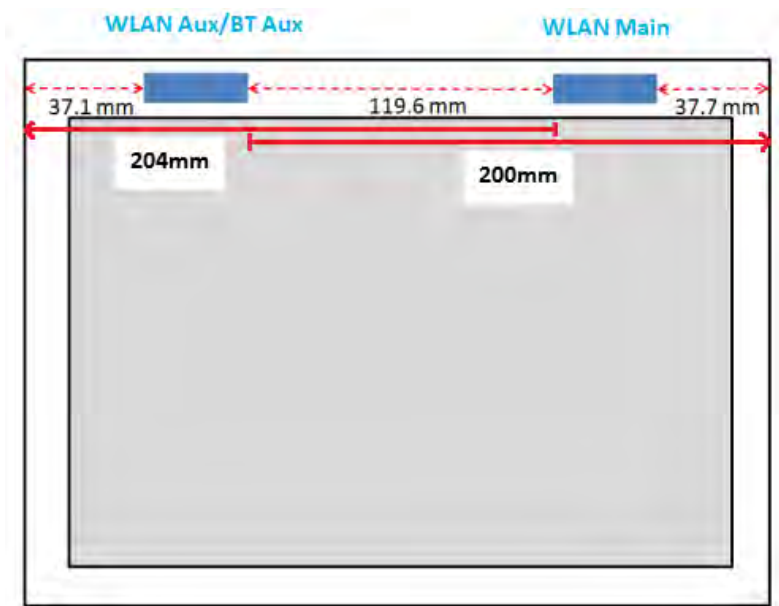
Fig.15 Antenna location (tablet mode, front view)
