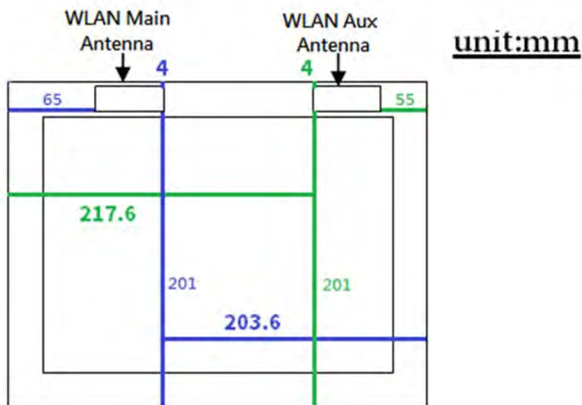
Fig.10 Antenna location of EUT (tablet mode)
