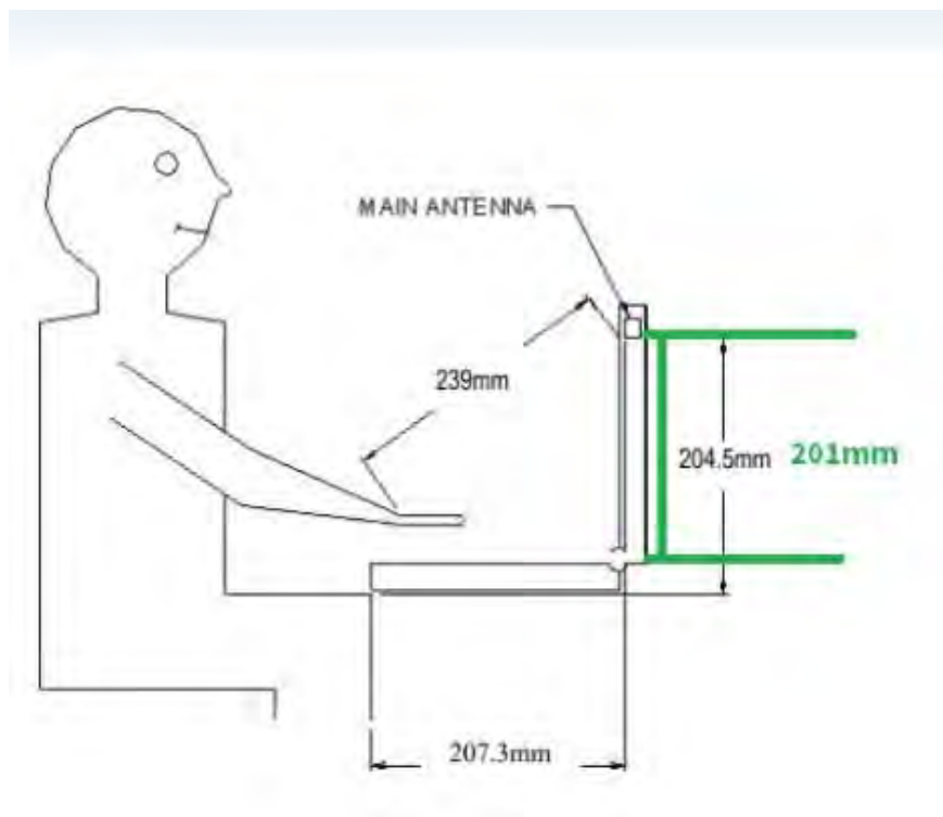
Fig.11 Antenna location of EUT (laptop mode)
