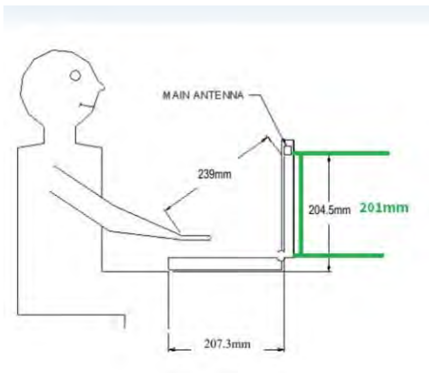
Fig.11 Antenna location of EUT (laptop mode)
