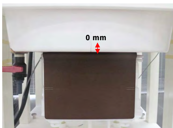
Fig.8 EUT (NB mode) Bottom side to flat phantom
