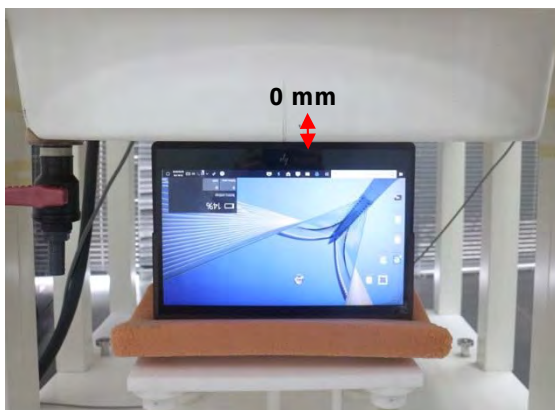
Fig.5 EUT (TB mode) Bottom side to flat phantom
