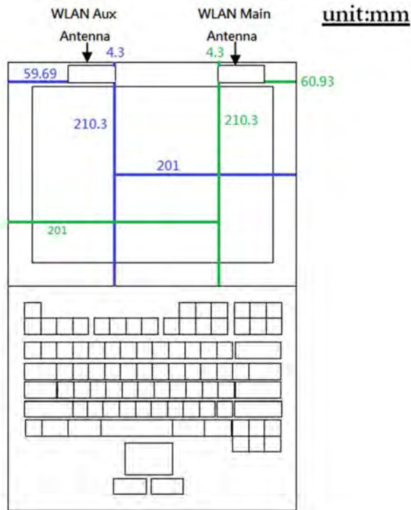
Antenna location (laptop mode)
