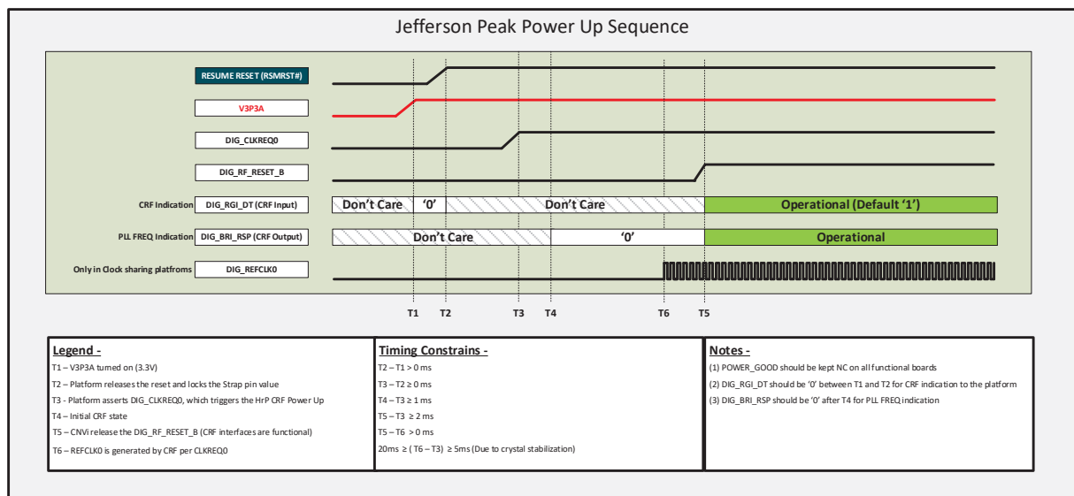
Figure 9–8 Jefferson Peak power-up sequence
