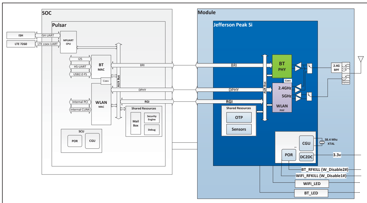
Figure 1–1 Jefferson Peak module block diagram
