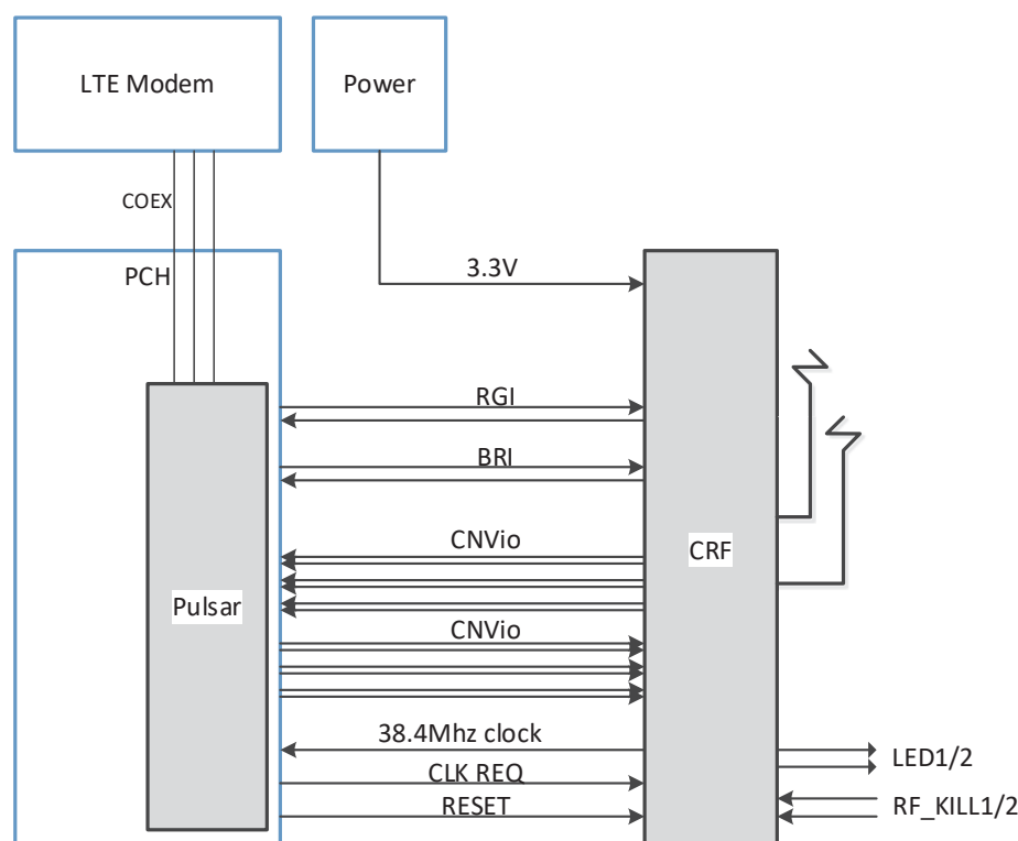
Figure 2–2 Jefferson Peak interfaces
