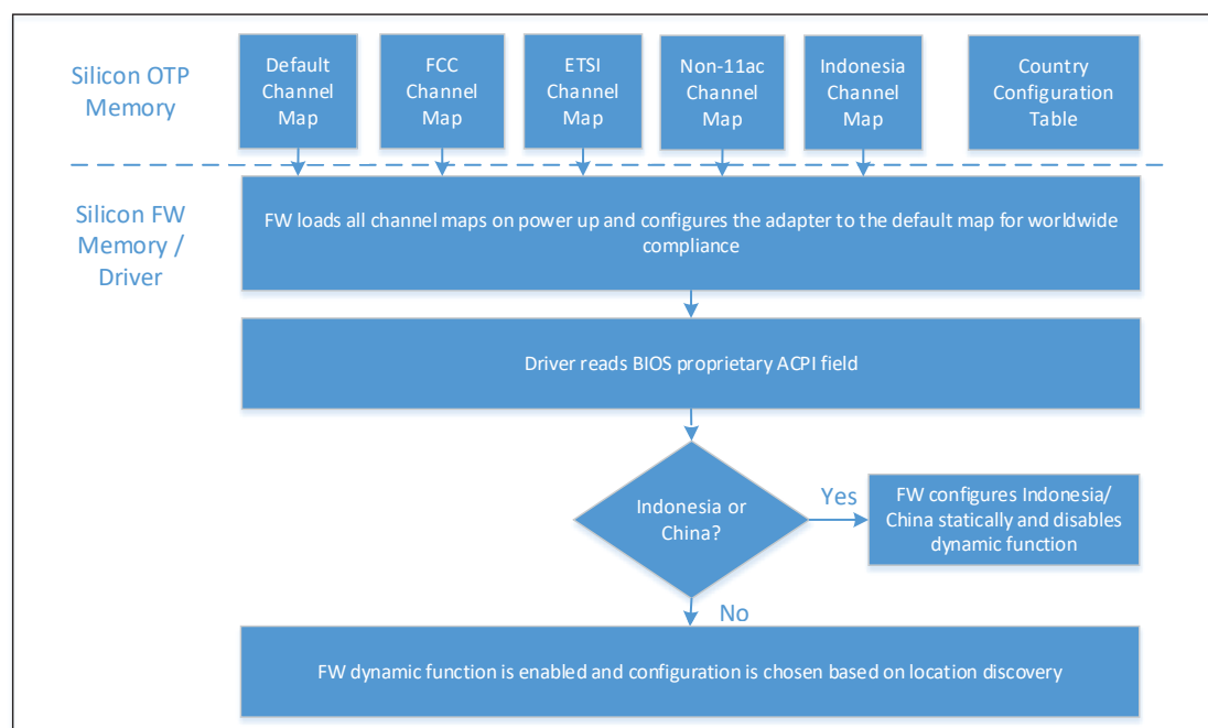
Figure 8–2 Dynamic regulatory architecture
