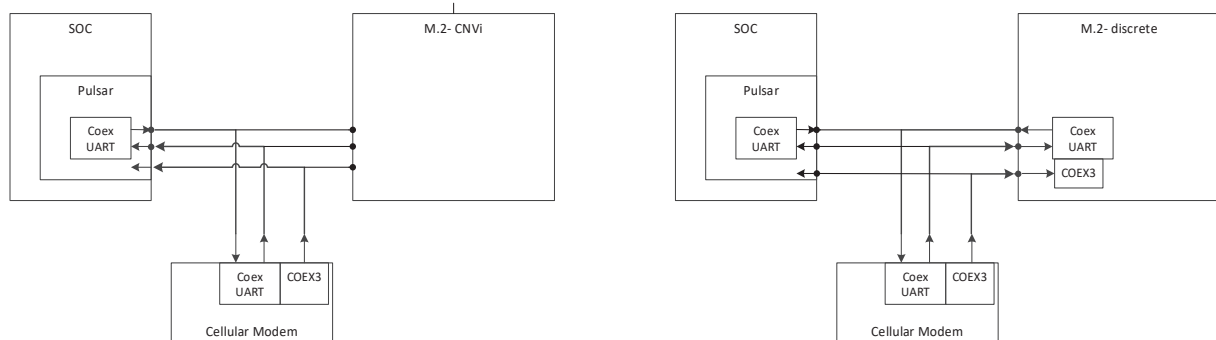
Figure 9–7 Coexistence UART for connectivity / modem 3-way configuration
