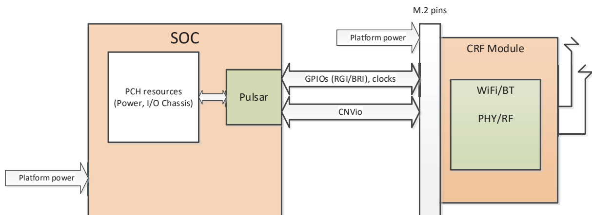
Figure 2–1 CNVi architecture
