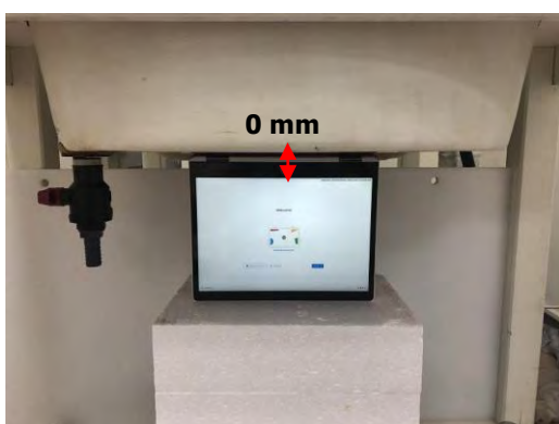
Fig.5 EUT Bottom side to flat phantom
