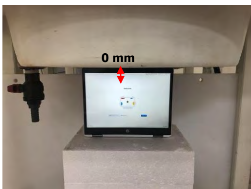
Fig.4 EUT Top side to flat phantom
