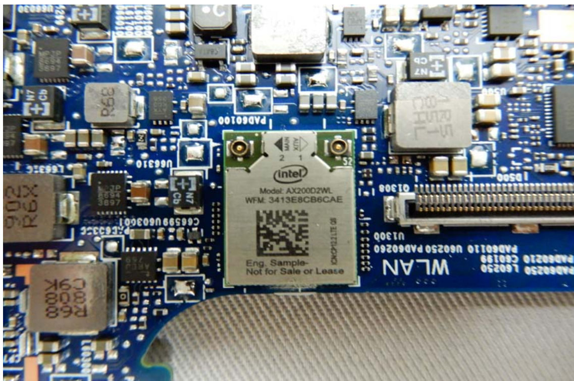
WLAN / BT Module-1 (Model No.: AX200D2WL)
