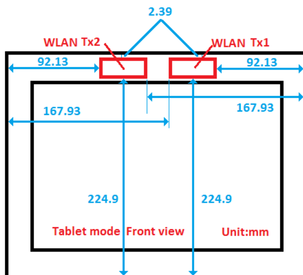
Fig.8 Antenna position of EUT (Tablet mode)
