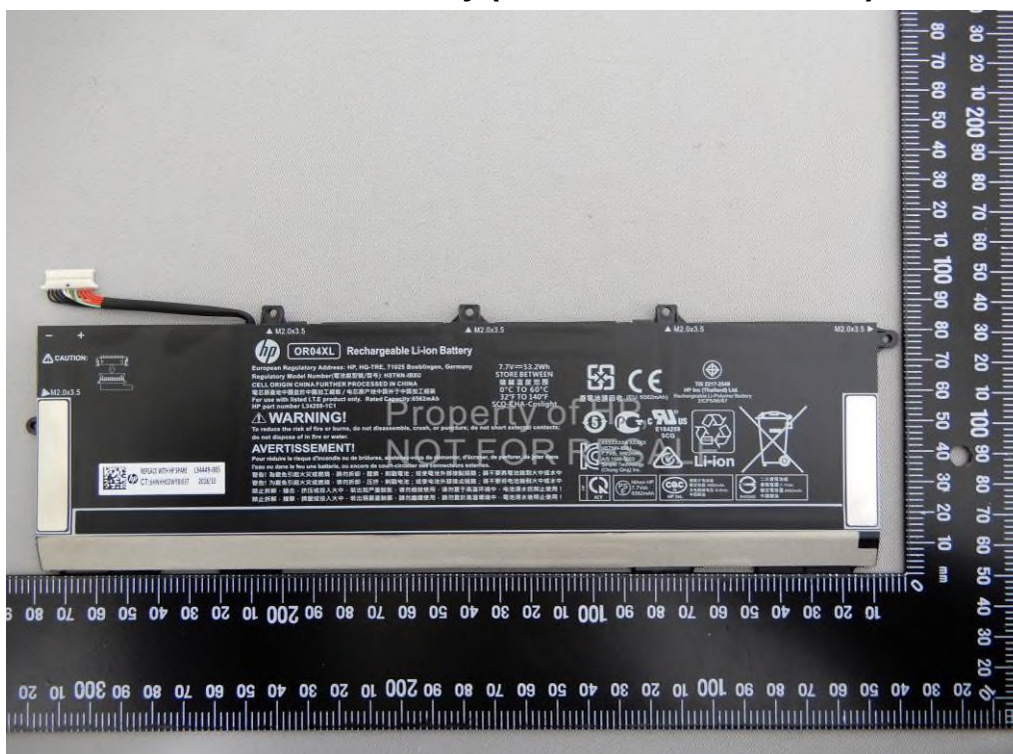
Front View of Battery (Model No.: HSTNN-IB8U)
