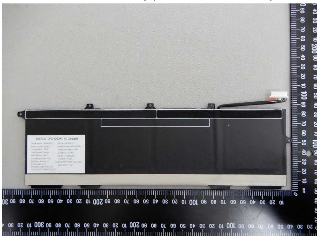
Back View of Battery (Model No.: HSTNN-IB8U)
