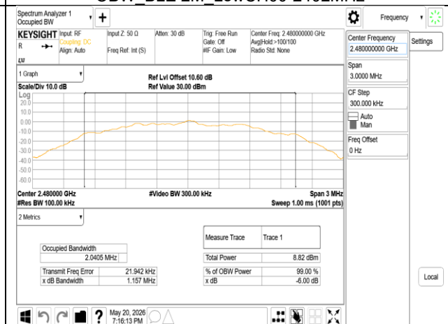
OBW_BLE 2M_HighCH39-2480MHz
