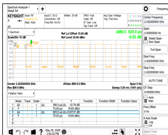
BLE_1M_LowCH00-2402
