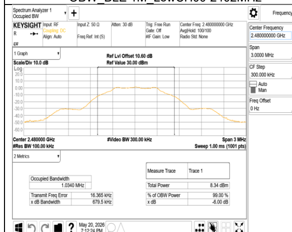
OBW_BLE 1M_HighCH39-2480MHz
