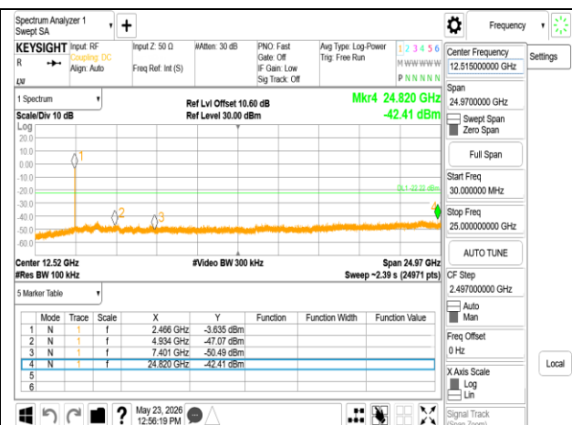
802.11g_20MHz_Chain0_2467MHz
