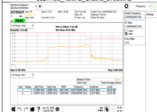
802.11be 40MHz Chain0_5835MHz_UNII 4
