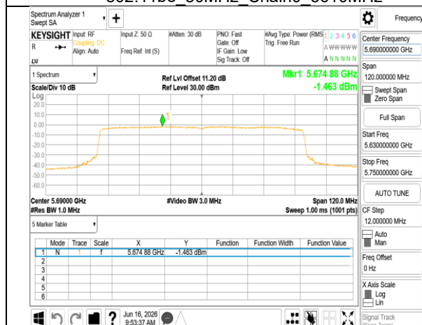
802.11be_80MHz_Chain0_5690MHz_UNII 2C
