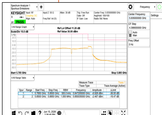
802.11n_40MHz_Chain0_5835MHz_UNII 4
