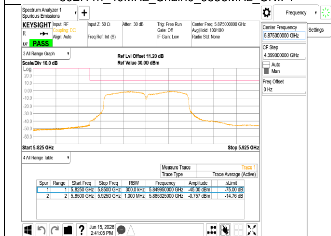
802.11n_40MHz_Chain0_5875MHz
