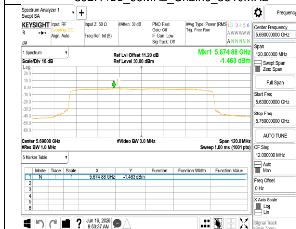
802.11be_80MHz_Chain0_5690MHz_UNII 2C
