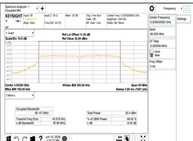
802.11n 40MHz Chain0_5835MHz
