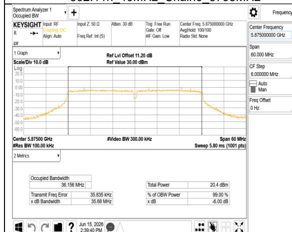
802.11n 40MHz Chain0_5875MHz
