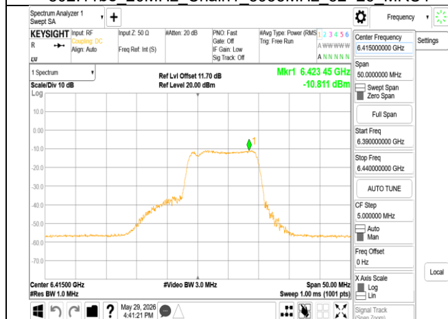
802.11be_20MHz_Chain1_6415MHz_106+26_MRUI
