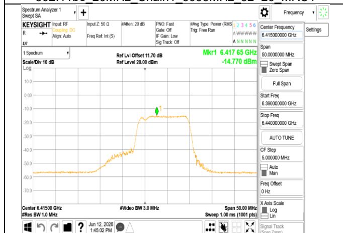
802.11be_20MHz_Chain1_6415MHz_106+26_MRU2
