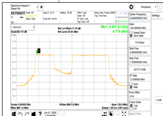
802.11be 80MHz Chain0 6945MHz 484+242 MRU2
