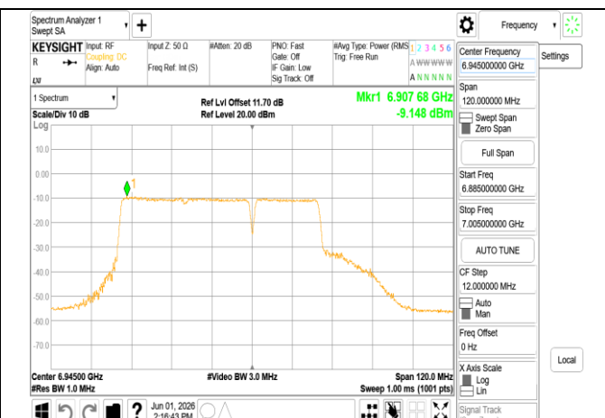
802.11be 80MHz Chain0 6945MHz 484+242 MRU4
