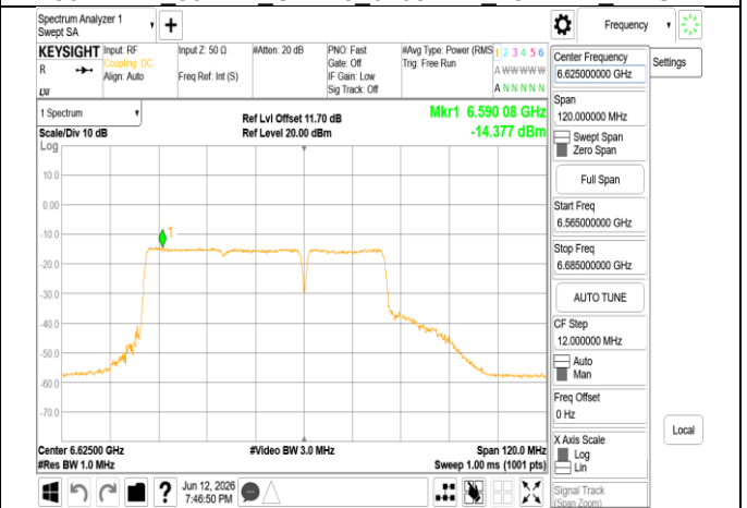
802.11be 80MHz Chain0_6625MHz 484+242 MRU4
