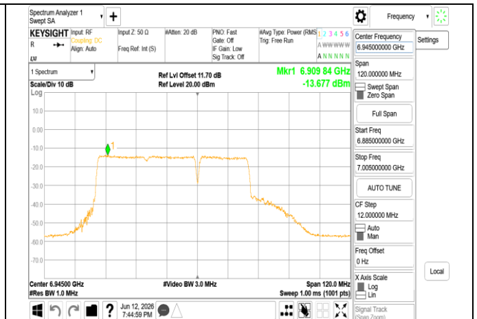
802.11be 80MHz Chain0 6945MHz 484+242 MRU4
