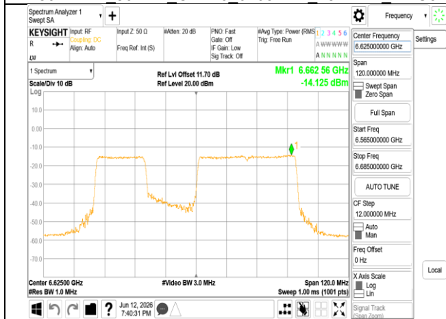
802.11be 80MHz Chain0_6625MHz 484+242 MRU2
