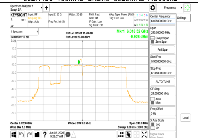
802.11be_160MHz_Chain0_6025MHz_996+484+242_MR1
