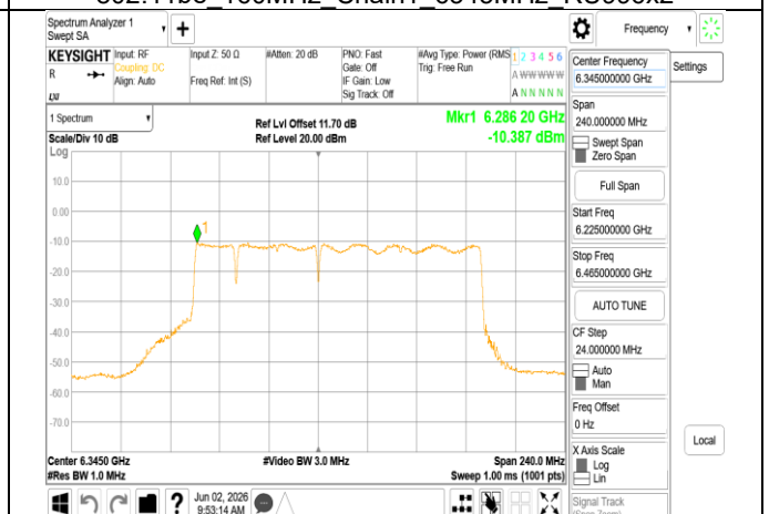
802.11be_160MHz_Chain1_6345MHz_996+484+242_MR1
