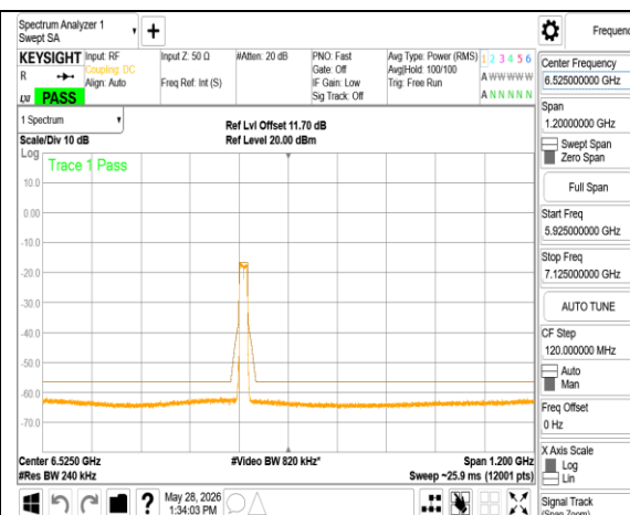
802.11ax_20MHz_Chain0_6415MHz RU242
