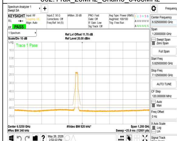
802.11ax_20MHz_Chain0_6475MHz
