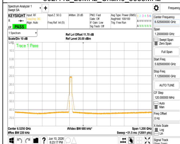
802.11a_20MHz_Chain0_6415MHz
