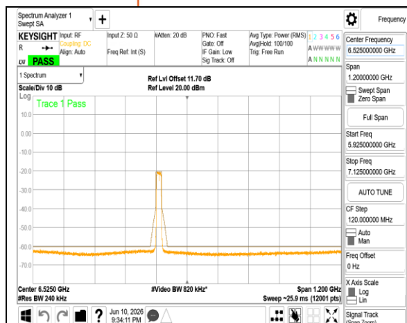
802.11ax_20MHz_Chain0_6415MHz
