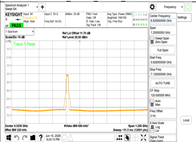
802.11a_20MHz_Chain1_6415MHz
