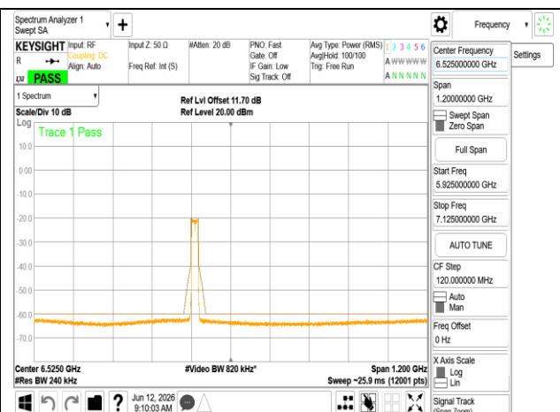
802.11ax_20MHz_Chain0_6415MHz RU242
