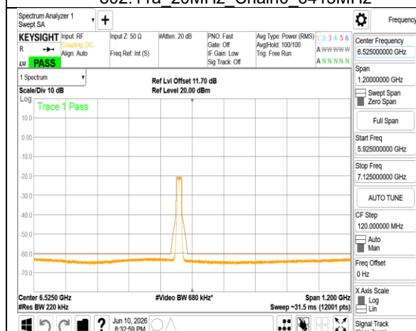
802.11a_20MHz_Chain0_6475MHz
