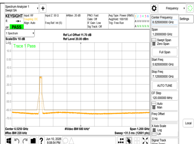
802.11a_20MHz_Chain0_6175MHz
