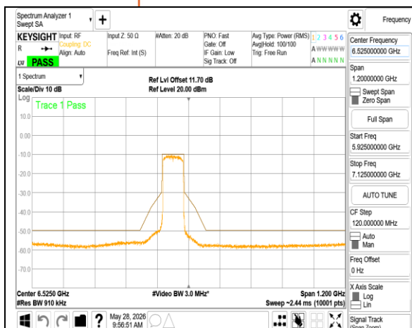
802.11ax_80MHz_Chain0_6465MHz
