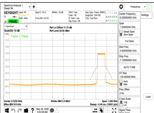
802.11ax 80MHz Chain0 6945MHz RU996
