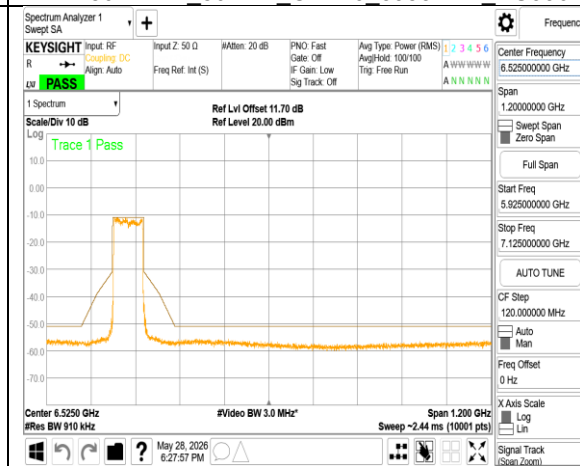
802.11ax_80MHz_Chain0_6145MHz RU996
