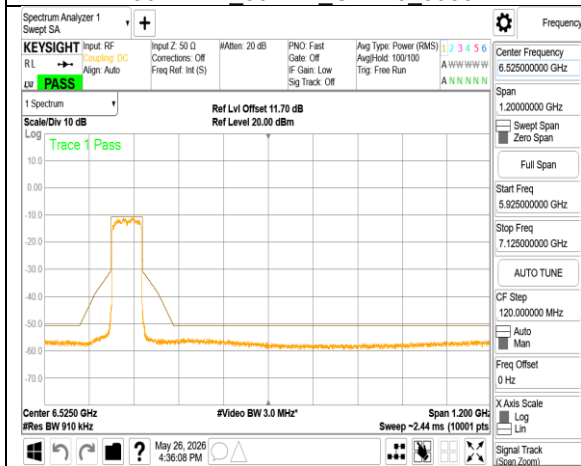
802.11ax_80MHz_Chain0_6145MHz
