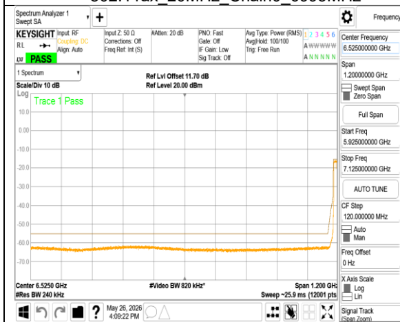
802.11ax_20MHz_Chain0_7115MHz
