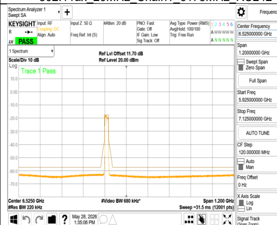
802.11ax_20MHz_Chain1_6415MHz RU242
