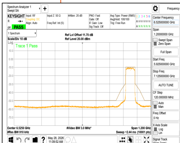
802.11ax 80MHz Chain0 6945MHz
