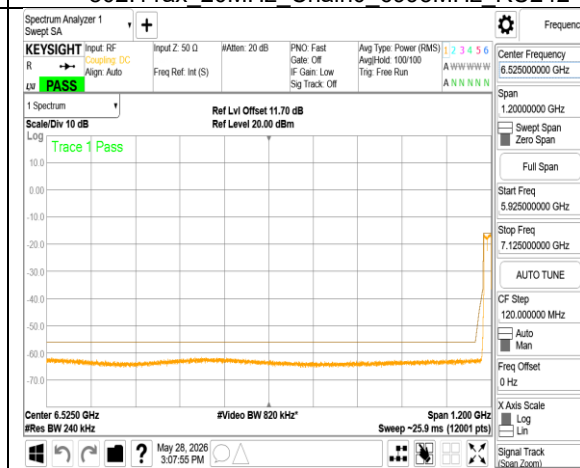
802.11ax_20MHz_Chain0_7115MHz RU242
