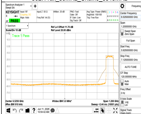
802.11ax_80MHz_Chain0_7025MHz
