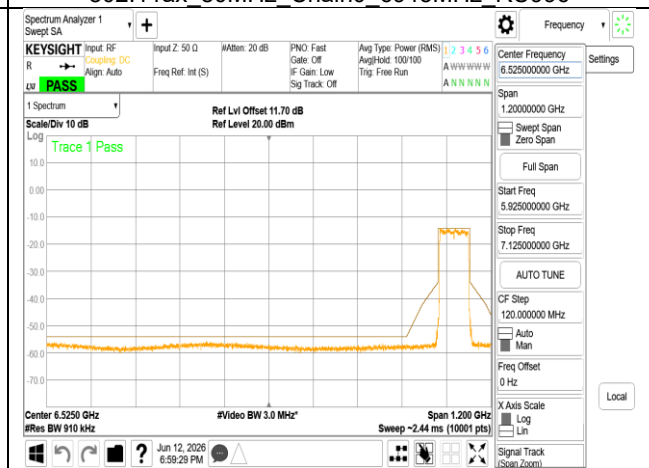
802.11ax_80MHz_Chain0_7025MHz RU996
