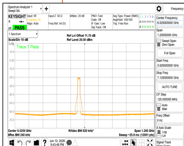
802.11ax_20MHz_Chain1_6475MHz
