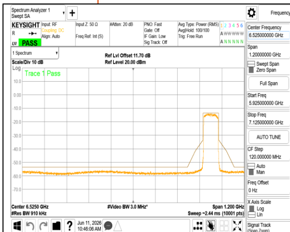
802.11ax_80MHz_Chain0_6945MHz
