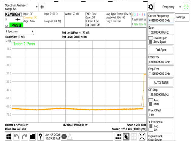
802.11ax_20MHz_Chain0_7115MHz RU242
