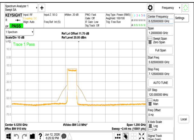
802.11ax_80MHz_Chain0_6465MHz RU996
