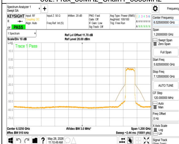
802.11ax_80MHz_Chain1_6945MHz
