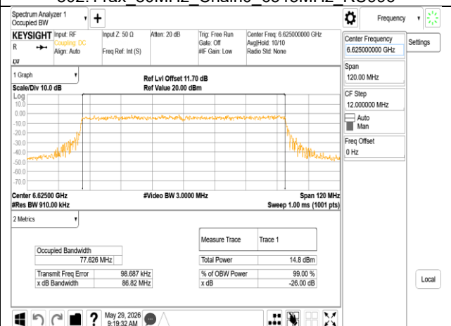
802.11ax_80MHz_Chain0_6625MHz RU996
