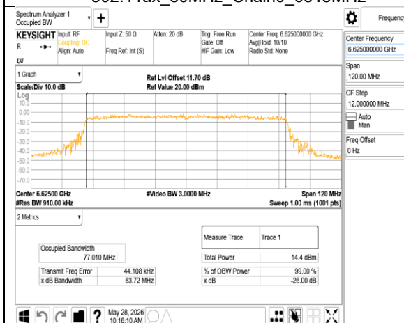
802.11ax_80MHz_Chain0_6625MHz
