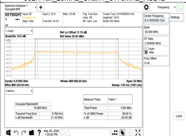
802.11ax_20MHz_Chain1_6415MHz RU242
