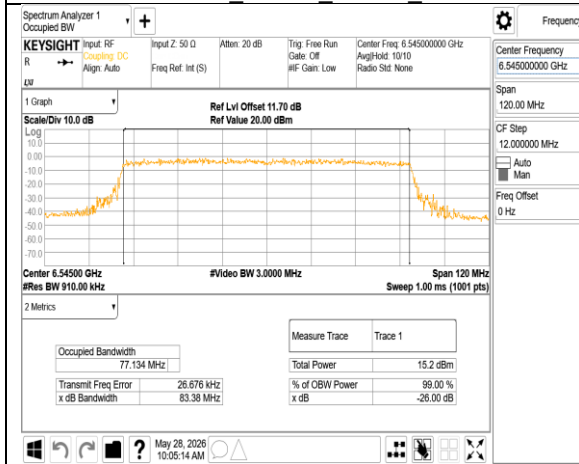
802.11ax_80MHz_Chain0_6545MHz
