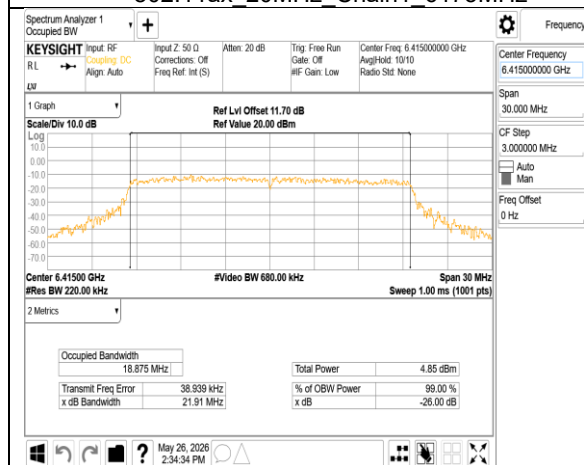
802.11ax_20MHz_Chain1_6415MHz
