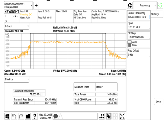
802.11ax_80MHz_Chain0_6545MHz RU996
