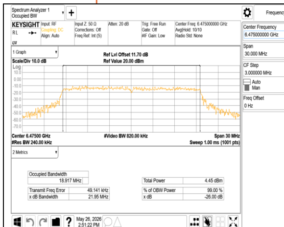
802.11ax_20MHz_Chain1_6475MHz
