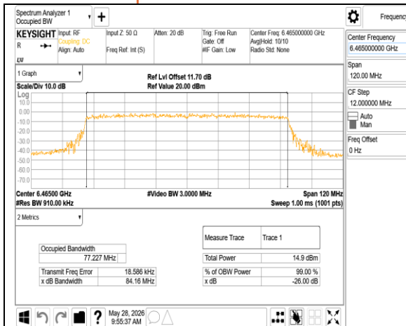
802.11ax_80MHz_Chain0_6465MHz
