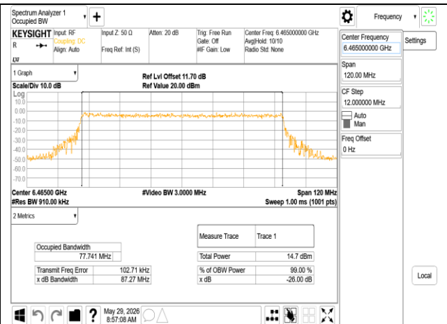
802.11ax_80MHz_Chain0_6465MHz RU996
