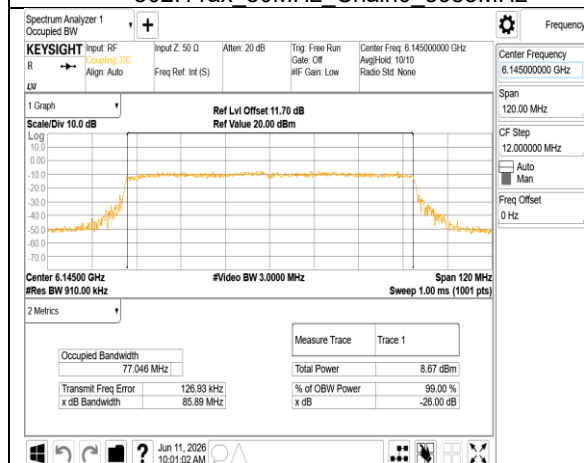
802.11ax_80MHz_Chain0_6145MHz
