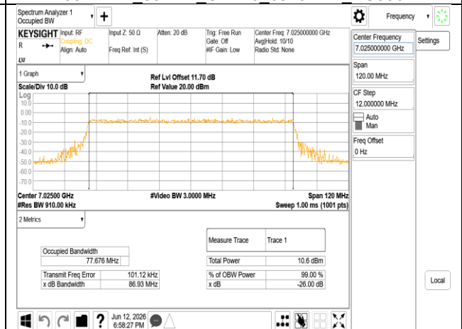
802.11ax 80MHz Chain0 7025MHz RU996
