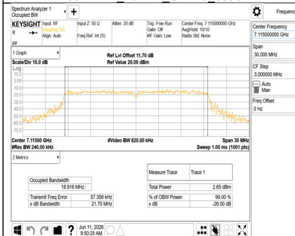
802.11ax_20MHz_Chain0_7115MHz
