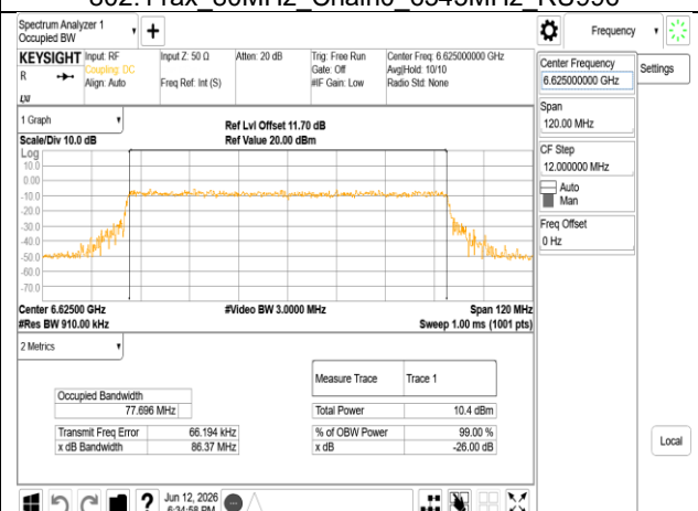
802.11ax_80MHz_Chain0_6625MHz RU996
