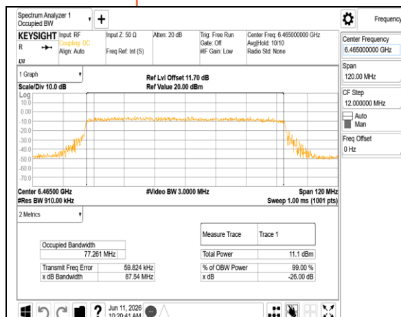
802.11ax_80MHz_Chain0_6465MHz
