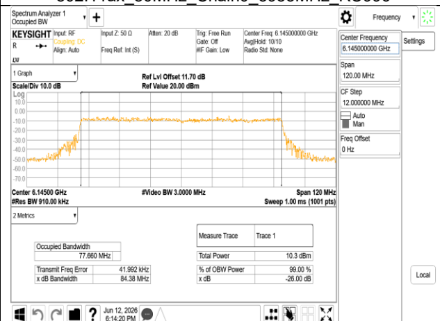
802.11ax_80MHz_Chain0_6145MHz RU996
