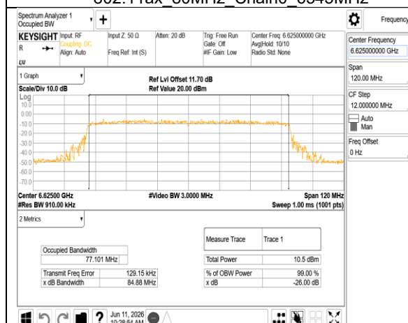
802.11ax_80MHz_Chain0_6625MHz
