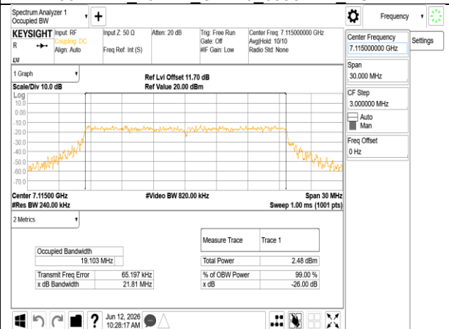
802.11ax_20MHz_Chain0_7115MHz RU242
