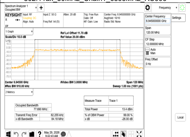
802.11ax_80MHz_Chain1_6945MHz RU996
