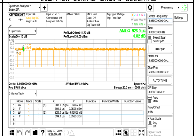
802.11ax 80MHz Chain0_5985MHz_RU996
