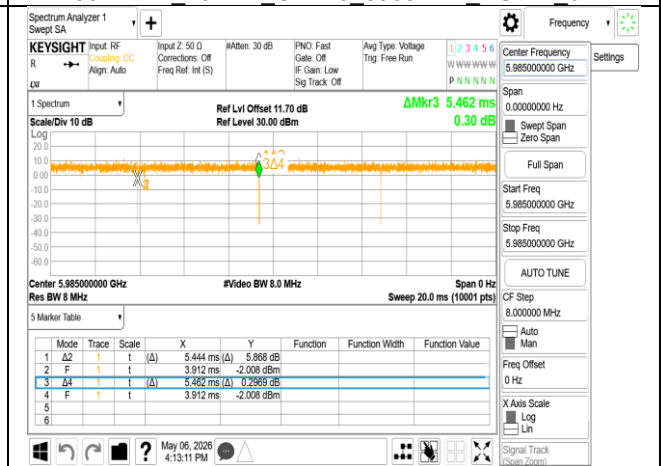
802.11ax 80MHz Chain0_5985MHz
