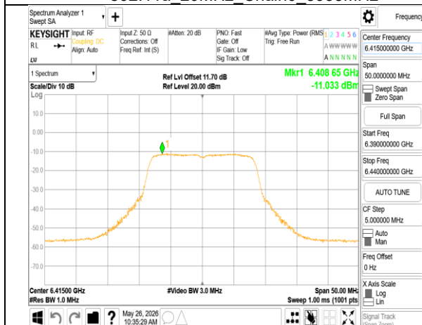
802.11a_20MHz_Chain0_6415MHz
