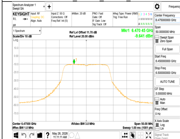
802.11a_20MHz_Chain0_6475MHz
