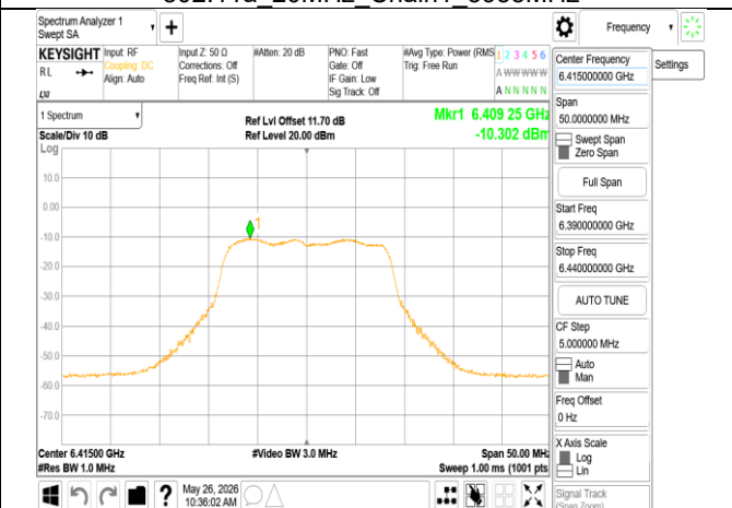
802.11a_20MHz_Chain1_6415MHz
