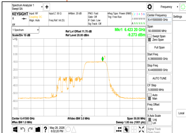
802.11ax 20MHz Chain0 6415MHz RU106_54
