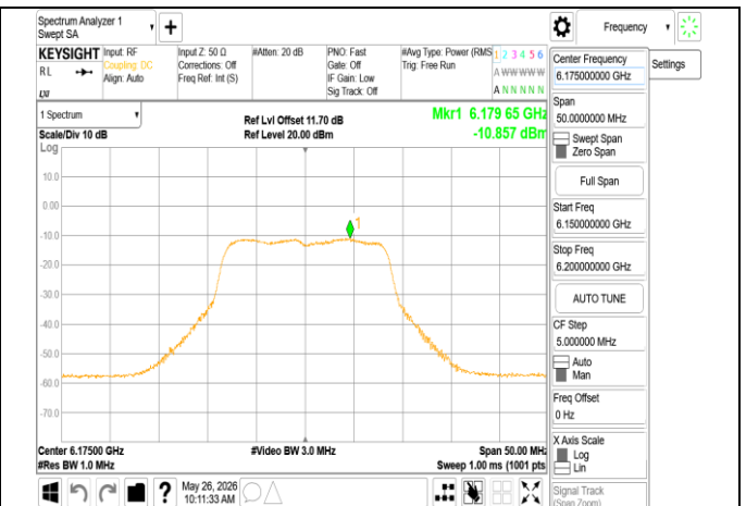
802.11a_20MHz_Chain0_6175MHz
