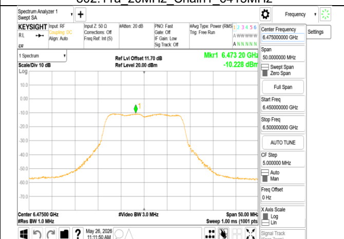
802.11a_20MHz_Chain1_6475MHz
