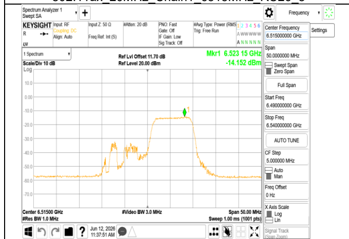
802.11ax 20MHz Chain1 6515MHz RU106_54
