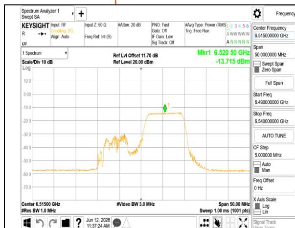
802.11ax 20MHz Chain0 6515MHz RU106_54
