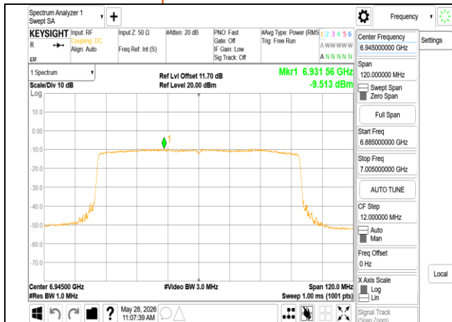
802.11ax_80MHz_Chain0_6945MHz
