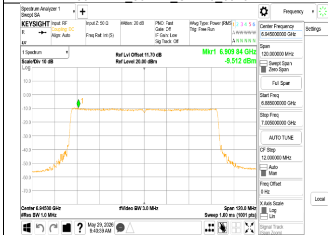
802.11ax_80MHz_Chain0_6945MHz_RU996
