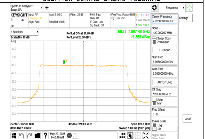
802.11ax_80MHz_Chain0_7025MHz_RU996
