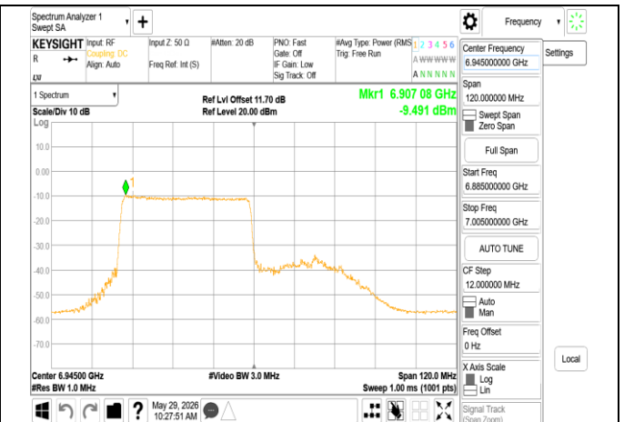
802.11ax_80MHz_Chain0_6945MHz_RU484_65
