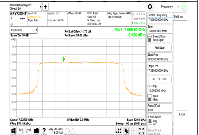
802.11ax_80MHz_Chain0_7025MHz
