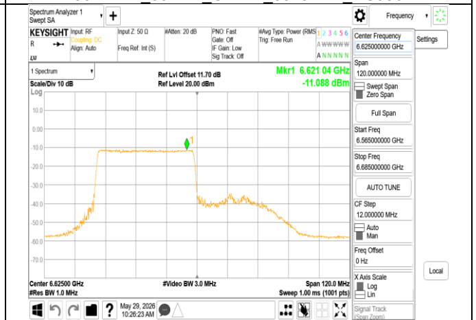
802.11ax 80MHz Chain1_6625MHz RU484_65
