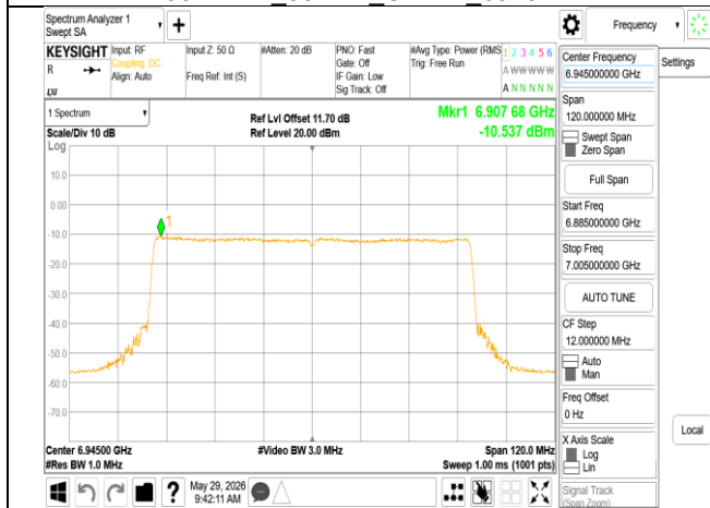
802.11ax 80MHz Chain1 6945MHz RU996
