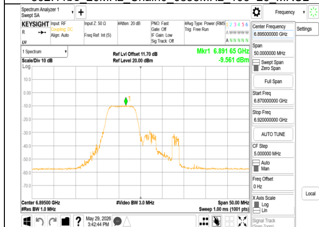
802.11be_20MHz_Chain0_6895MHz_52+26_MR01
