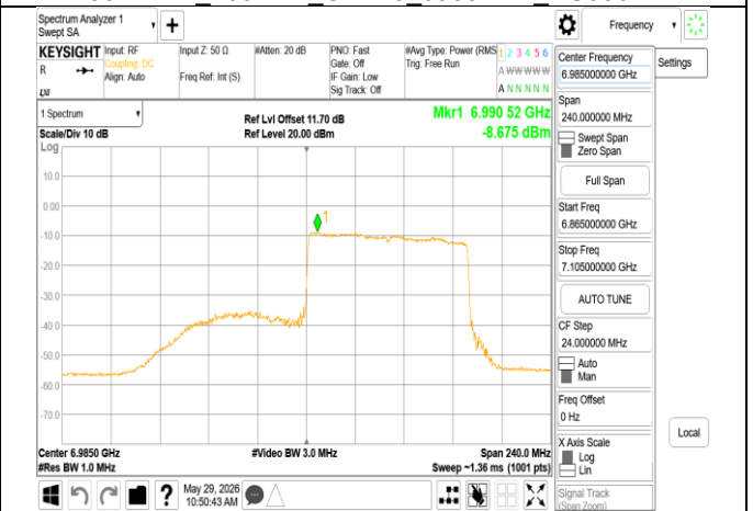
802.11ax_160MHz_Chain0_6985MHz_RU996_S67
