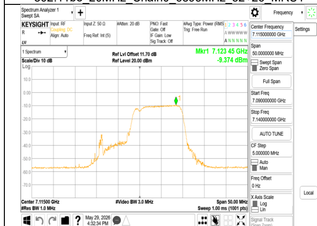
802.11be_20MHz_Chain0_7115MHz_106+26_MR02
