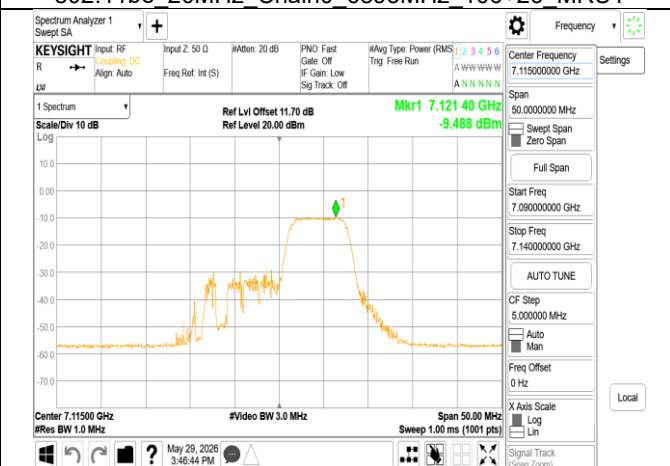
802.11be_20MHz_Chain0_7115MHz_52+26_MR03
