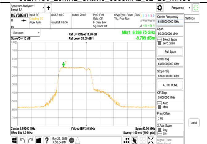
802.11be_20MHz_Chain0_6895MHz_106+26_MR01
