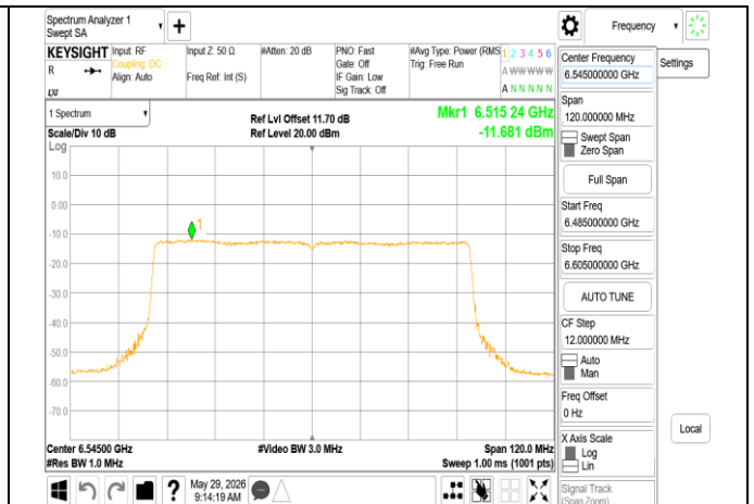
802.11ax 80MHz Chain1_6545MHz RU996
