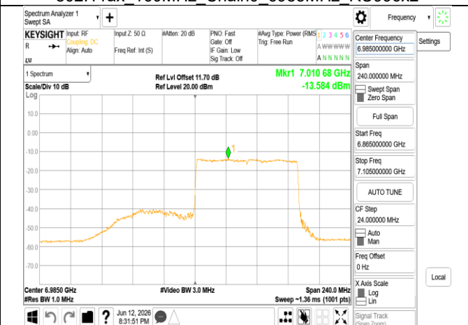
802.11ax_160MHz_Chain0_6985MHz_RU996_S67
