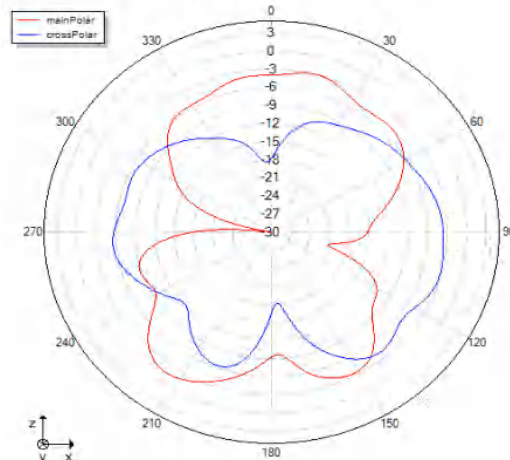
Phi=0 freq=2422MHz
