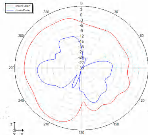
Phi=90 freq=2428MHz
