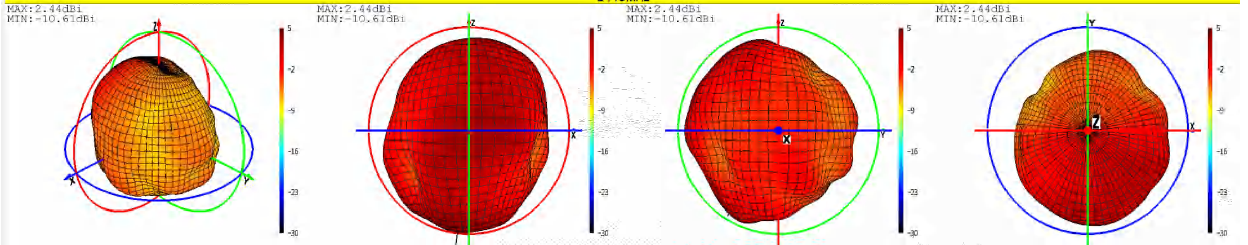
Phi=0 freq=2440MHz
