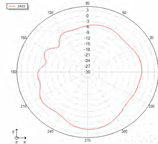
Theta=90 freq=2422MHz
