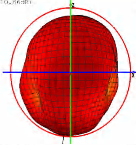
Phi=0 freq=2446MHz
