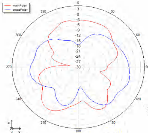
Phi=0 freq=2446MHz
