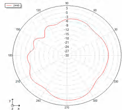
Theta=90 freq=2440MHz
