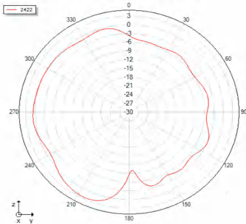
Phi=90 freq=2422MHz
