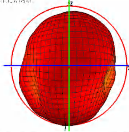
Phi=0 freq=2428MHz
