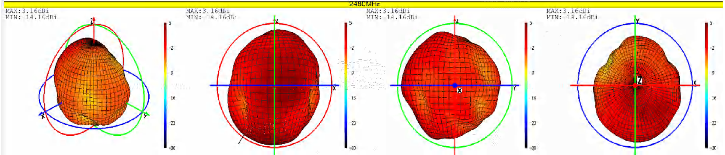
Phi=0 freq=2480MHz
