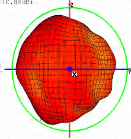
Theta=90 freq=2446MHz
