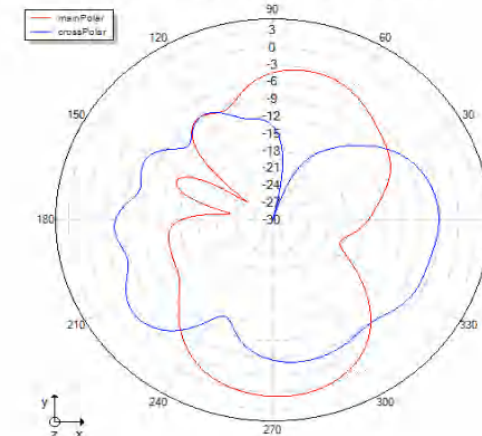
Theta=90 freq=2446MHz
