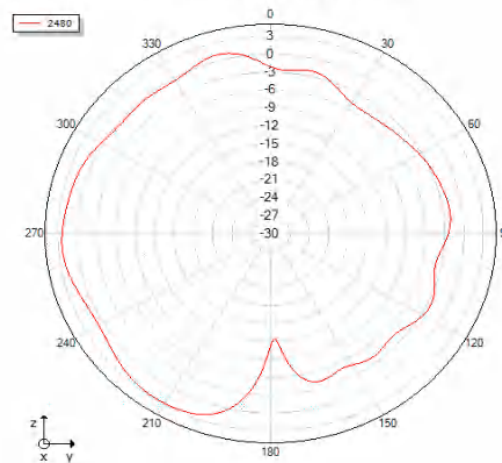
Phi=90 freq=2480MHz
