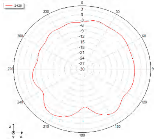
Phi=0 freq=2428MHz
