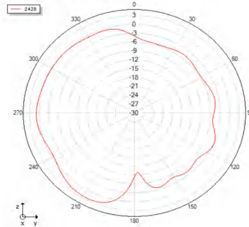
Phi=90 freq=2428MHz
