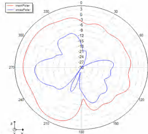
Phi=90 freq=2446MHz
