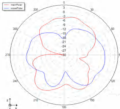
Phi=0 freq=2428MHz
