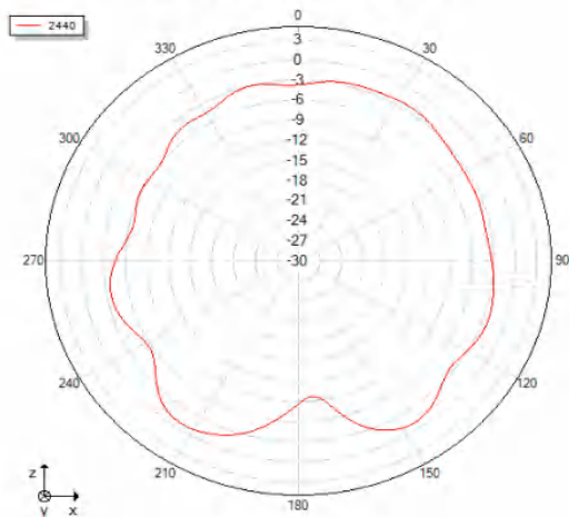
Phi=0 freq=2440MHz
