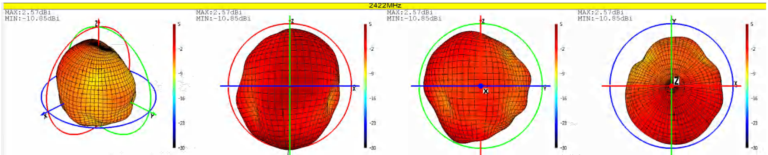
Phi=0 freq=2422MHz
