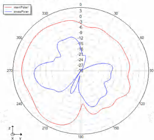
Phi=90 freq=2440MHz
