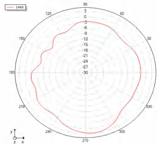
Theta=90 freq=2480MHz
