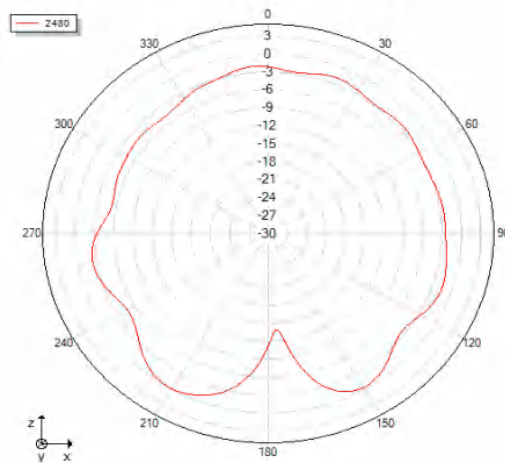
Phi=0 freq=2480MHz
