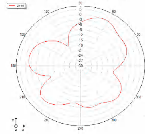
Theta=90 freq=2440MHz
