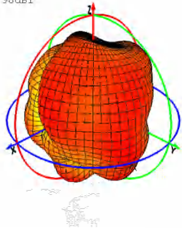
Phi=0 freq=2434MHz
