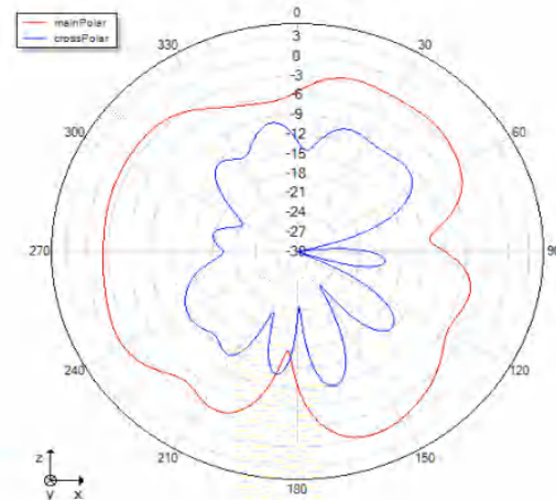
Phi=0 freq=2440MHz
