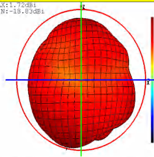
Phi=0 freq=2472MHz
