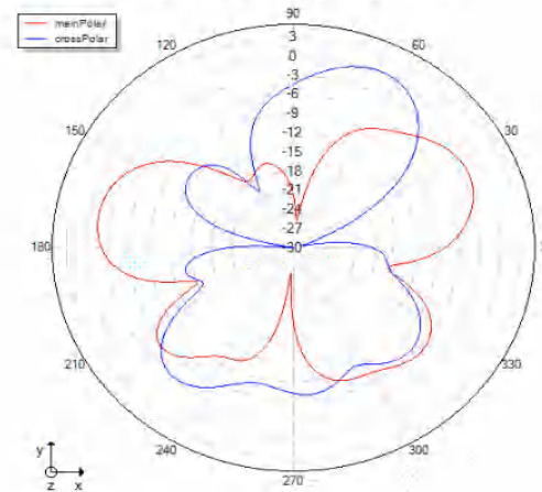
Theta=90 freq=2454MHz
