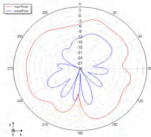
Phi=0 freq=2472MHz
