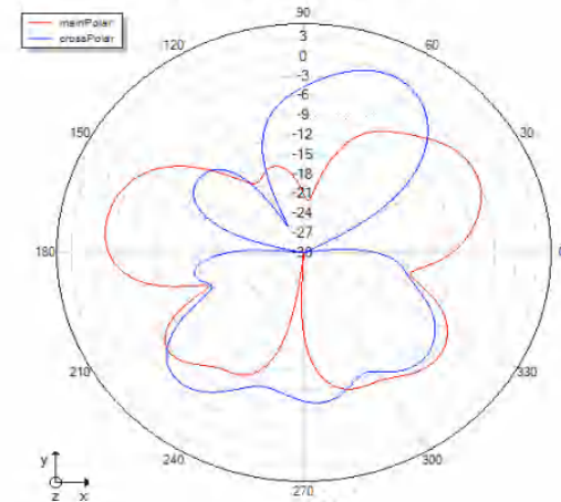
Theta=90 freq=2440MHz
