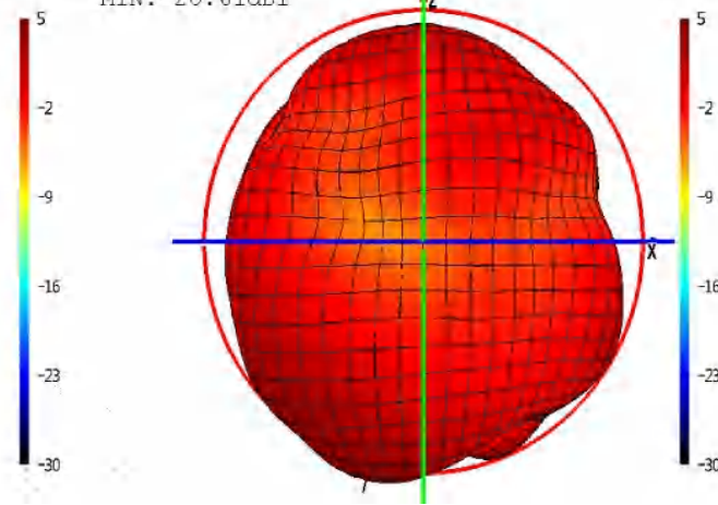
Phi=0 freq=2454MHz
