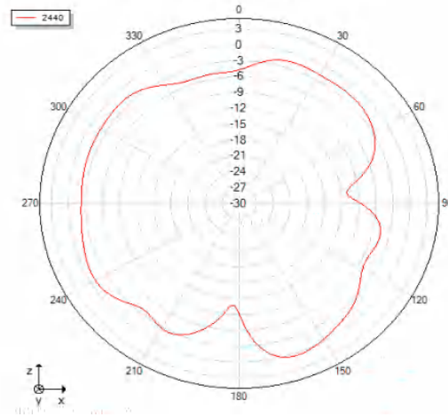
Phi=0 freq=2440MHz
