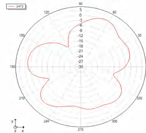
Theta=90 freq=2472MHz
