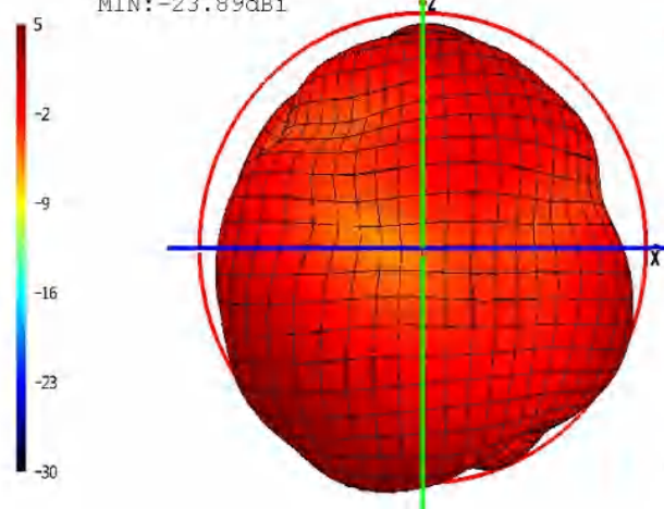
Phi=0 freq=2440MHz
