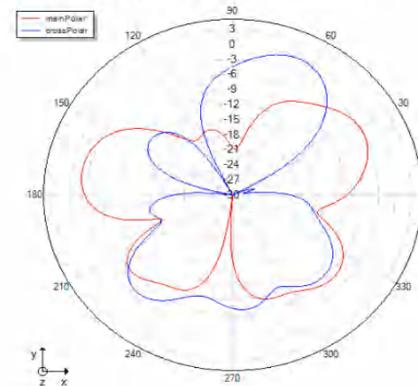
Theta=90 freq=2434MHz
