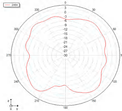
Phi=90 freq=2454MHz
