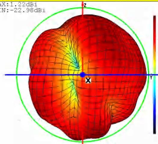
Theta=90 freq=2434MHz
