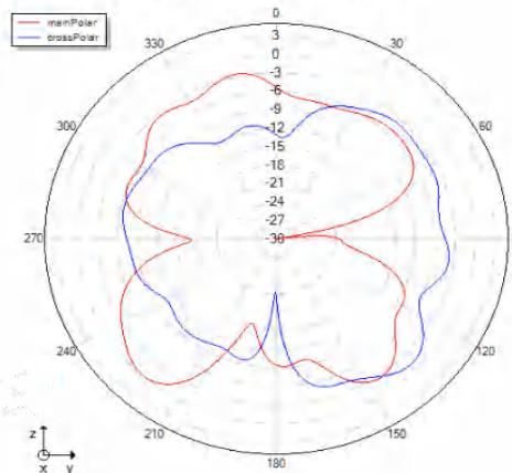
Phi=90 freq=2434MHz
