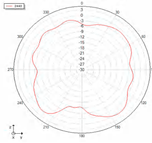
Phi=90 freq=2440MHz
