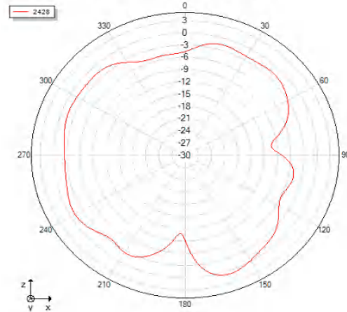
Phi=0 freq=2428MHz
