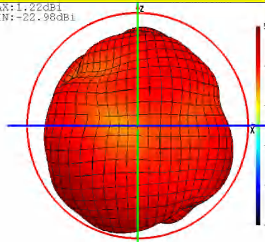
Phi=0 freq=2434MHz
