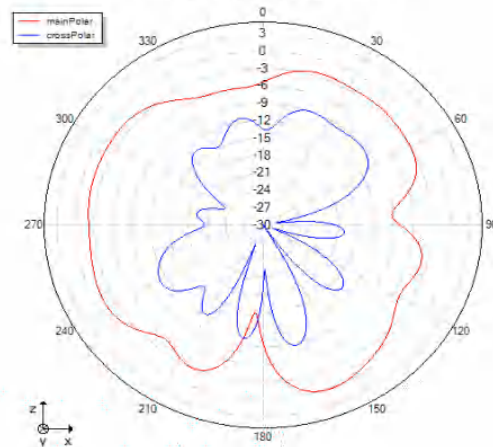
Phi=0 freq=2454MHz
