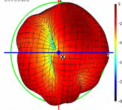
Theta=90 freq=2454MHz
