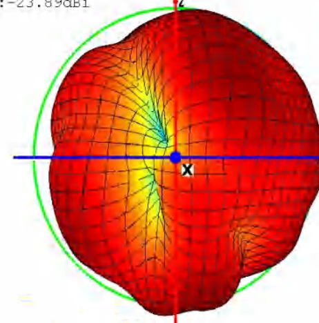
Phi=90 freq=2440MHz
