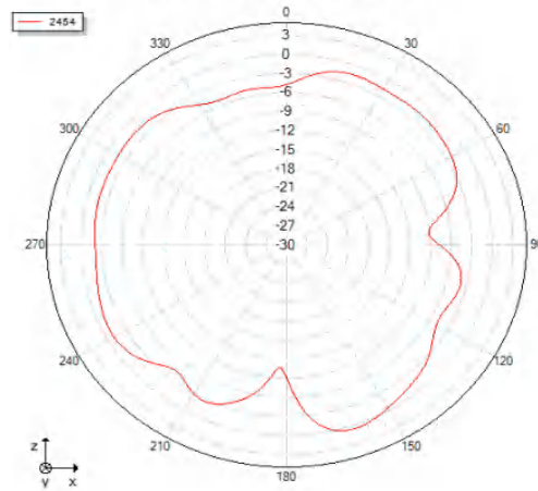
Phi=0 freq=2454MHz
