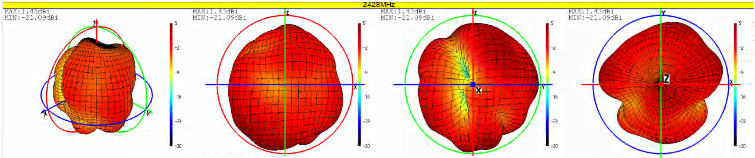
Phi=0 freq=2428MHz
