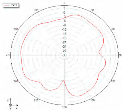
Phi=0 freq=2472MHz
