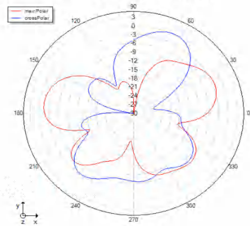
Theta=90 freq=2472MHz
