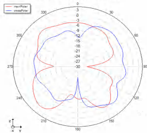
Phi=90 freq=2472MHz
