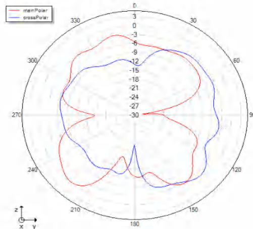
Phi=90 freq=2440MHz
