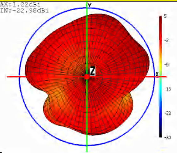
Theta=90 freq=2434MHz
