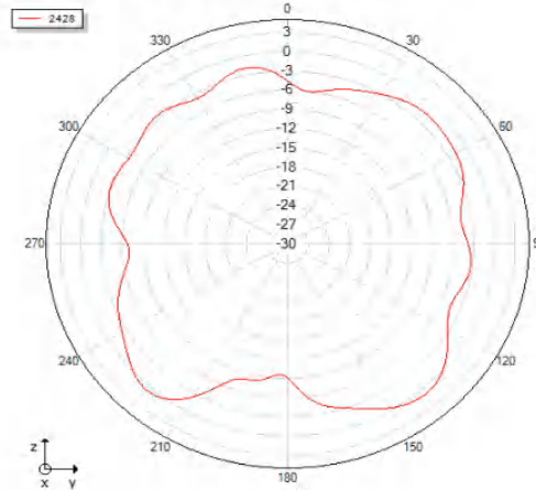
Phi=90 freq=2428MHz
