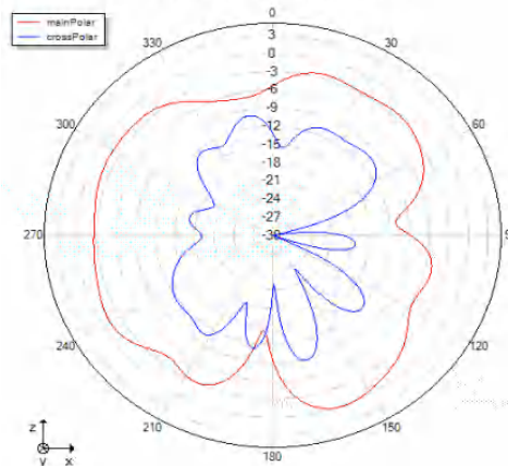
Phi=0 freq=2434MHz
