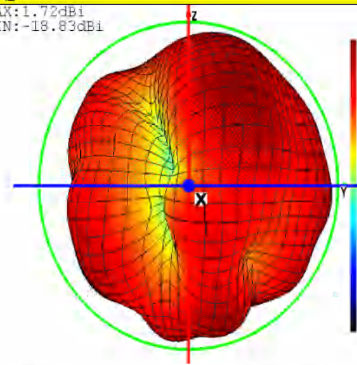
Theta=90 freq=2472MHz
