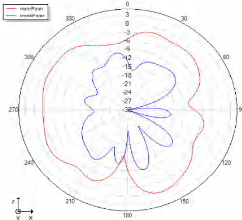
Phi=0 freq=2428MHz
