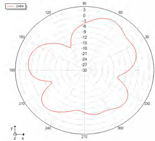
Theta=90 freq=2454MHz
