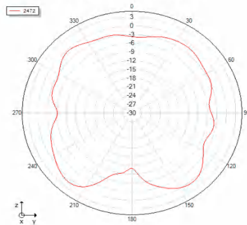
Phi=90 freq=2472MHz
