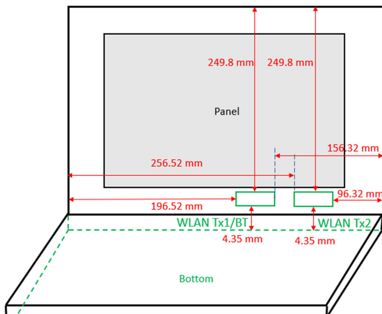
Photograph 5. Antenna position of EUT
