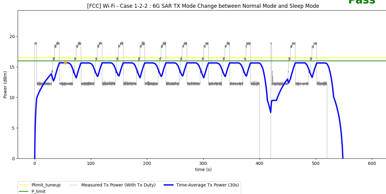
Figure 7-2 Time-averaged conducted TX power over time for test scenario 1-2-2
