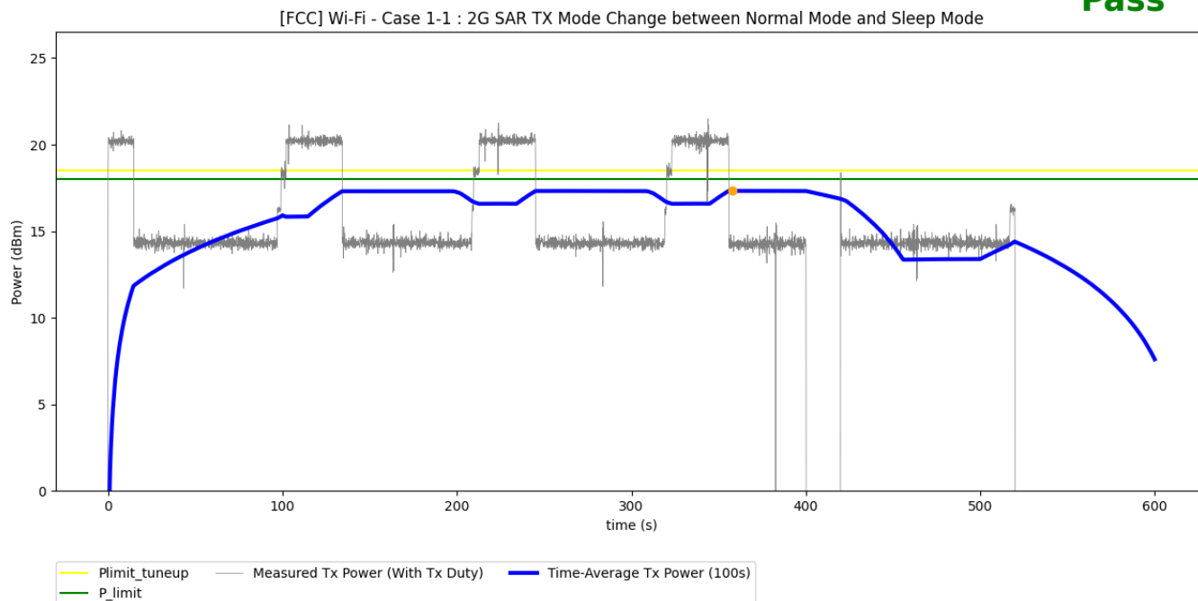
Figure 7-1 Time-averaged conducted TX power over time for test scenario 1-1
