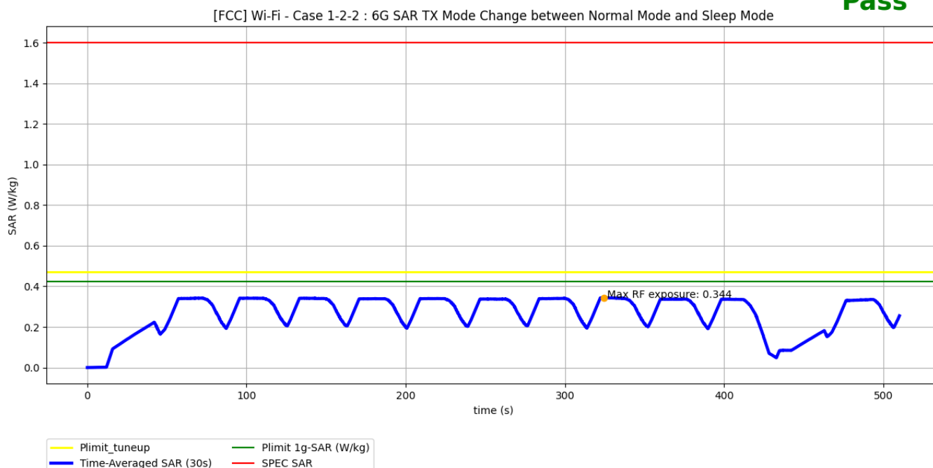
Figure 8-2 Time-averaged SAR measurement for scenario 1-2-2
