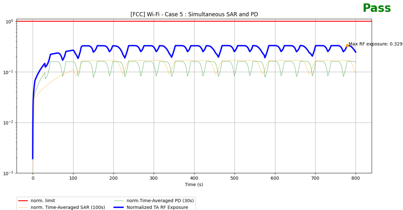
Figure 7-10 Normalized Time-averaged SAR over time for test scenario 5
