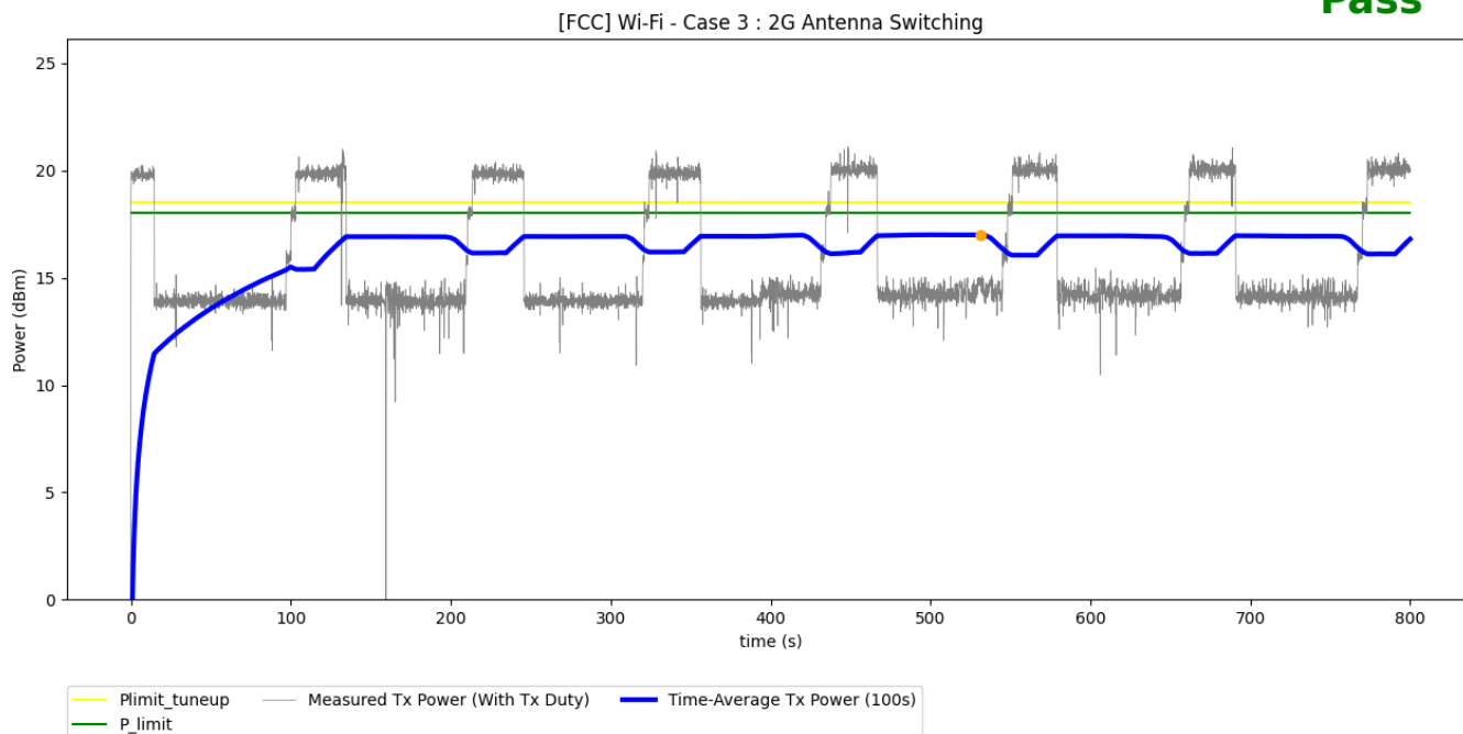
Figure 7-5 Time-averaged conducted TX power over time for test scenario 3
