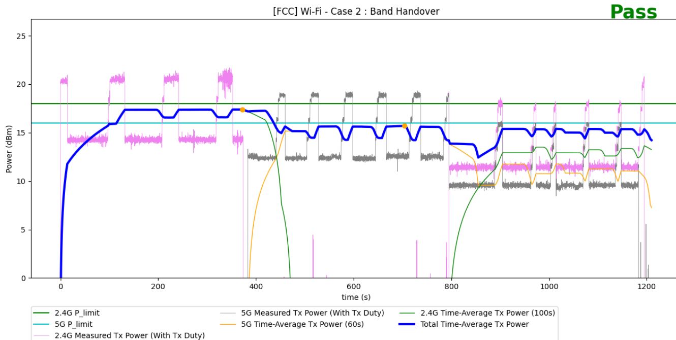
Figure 7-3 Time-averaged conducted TX power over time for test scenario 2
