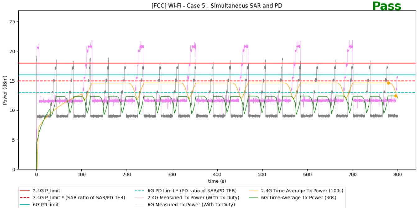
Figure 7-9 Time-averaged conducted TX power over time for test scenario 5
