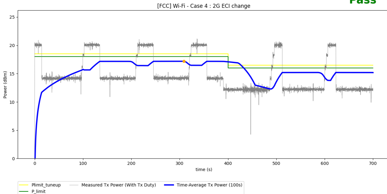
Figure 7-7 Time-averaged conducted TX power over time for test scenario 4
