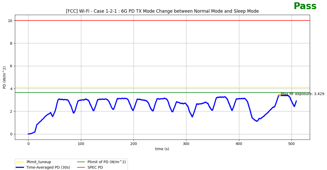
Figure 10-1 Time-averaged PD measurement for scenario 1-2-1
