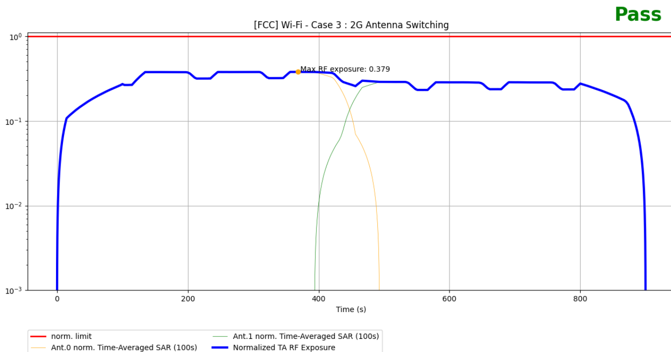
Figure 7-6 Normalized time-averaged SAR over time for test scenario 3
