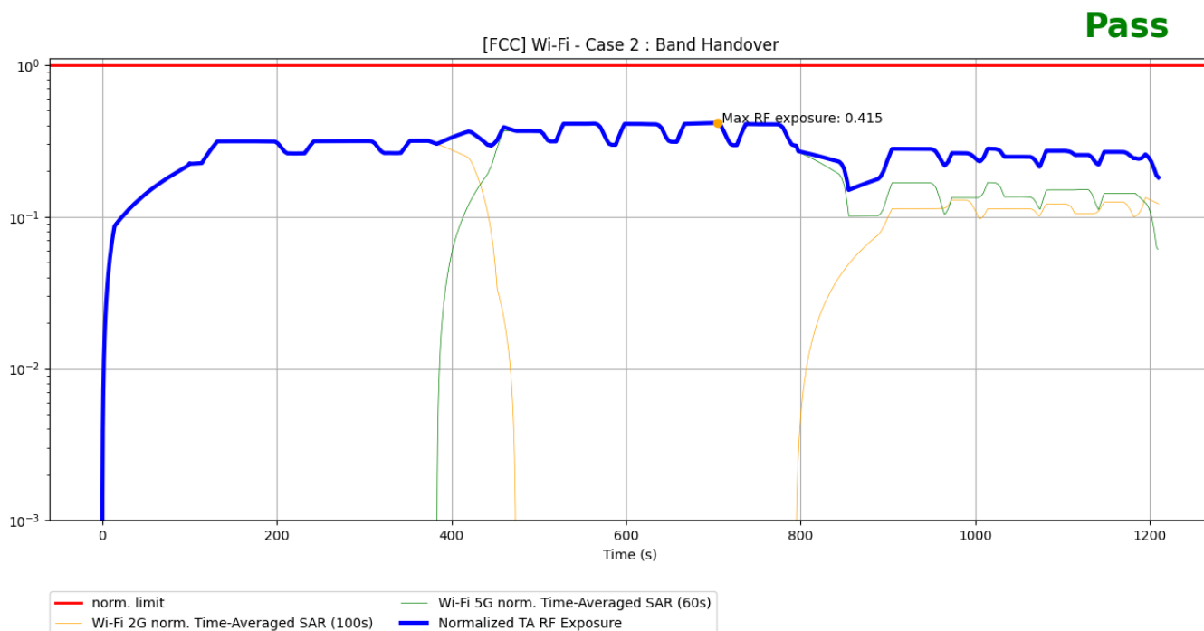
Figure 7-4 Normalized time-averaged SAR over time for test scenario 2
