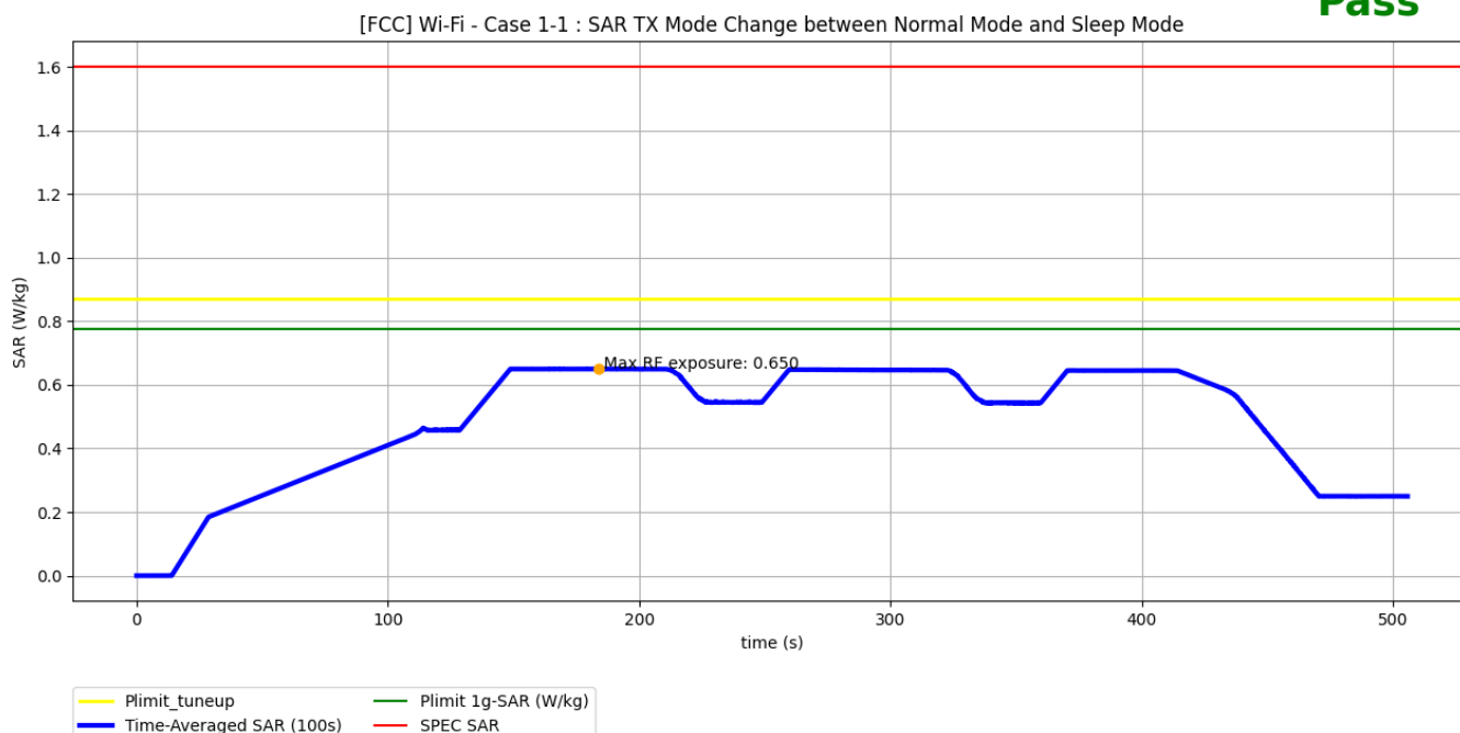
Figure 8-1 Time-averaged SAR measurement for scenario 1-1
