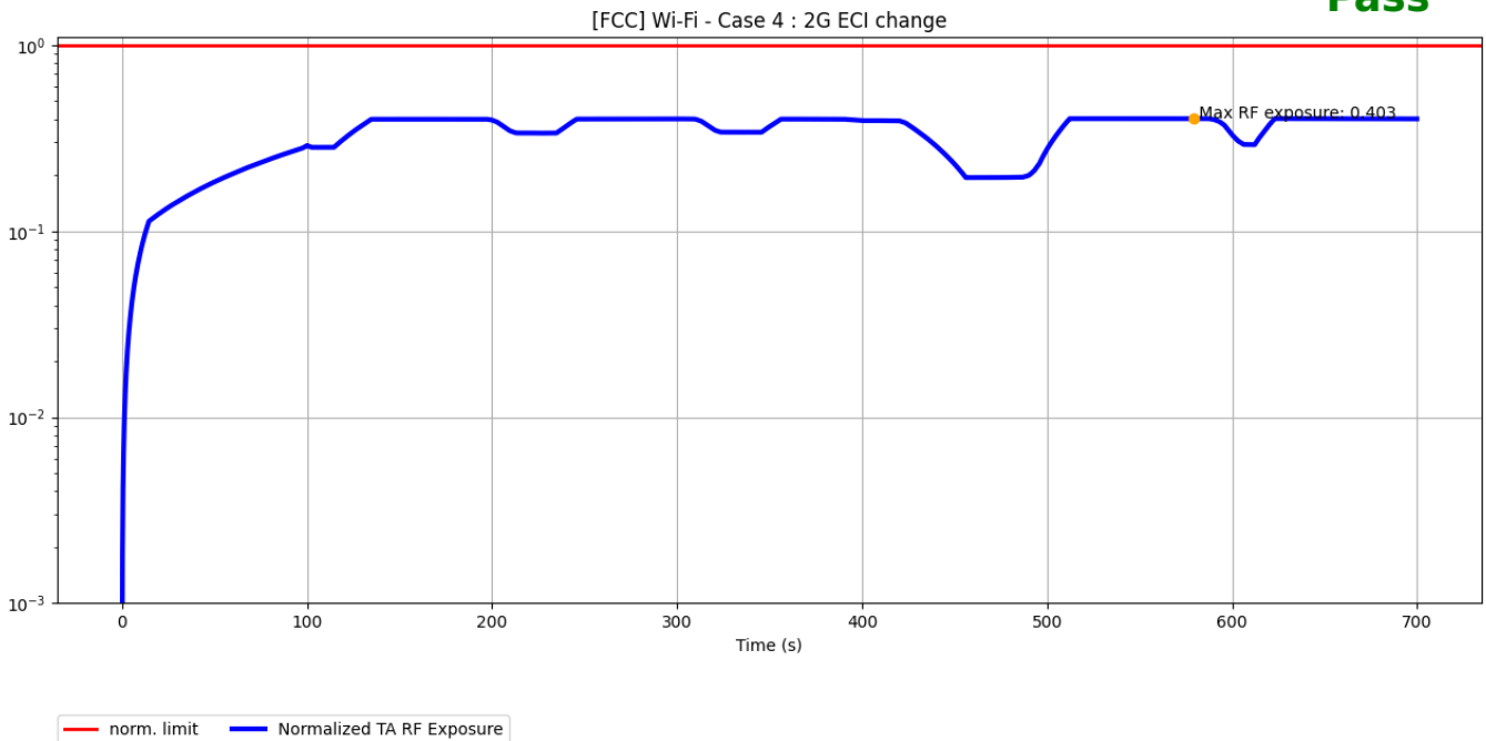
Figure 7-8 Time-averaged SAR over time for test scenario 4
