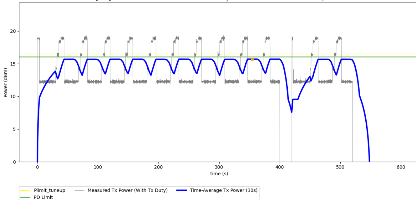
Figure 9-1 Time-averaged conducted TX power over time for test scenario 1-2-1
