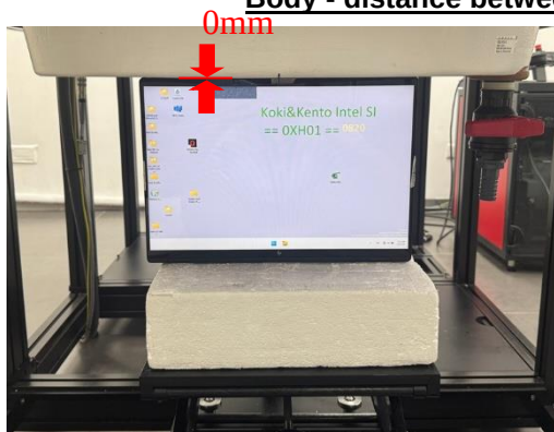
Photograph 1. Body, Top Edge, 0mm
