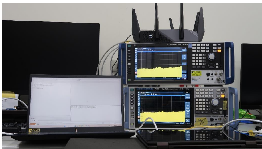
Conducted Setup Photo
