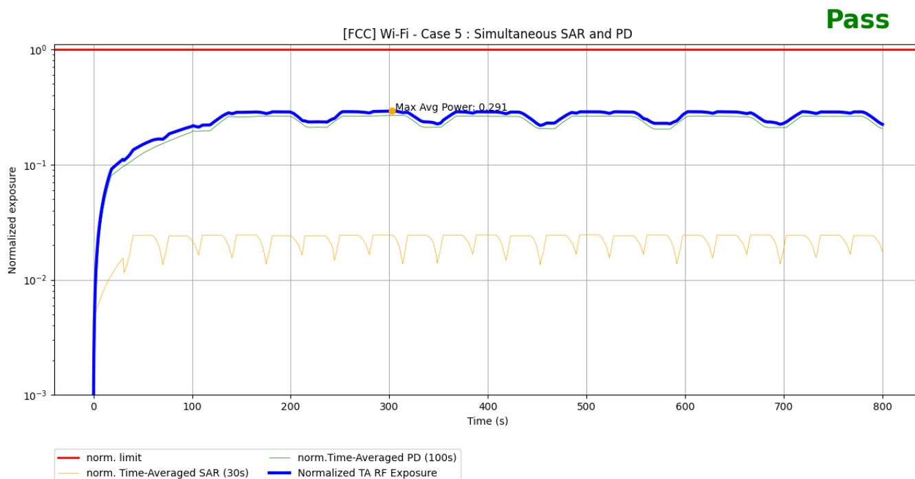
Figure 7-8 Normalized Time-averaged SAR over time for test scenario 5
