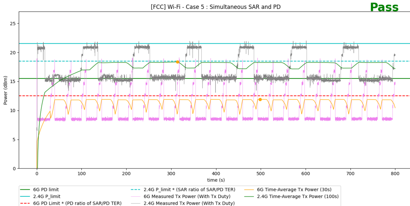
Figure 7-7 Time-averaged conducted TX power over time for test scenario 5
