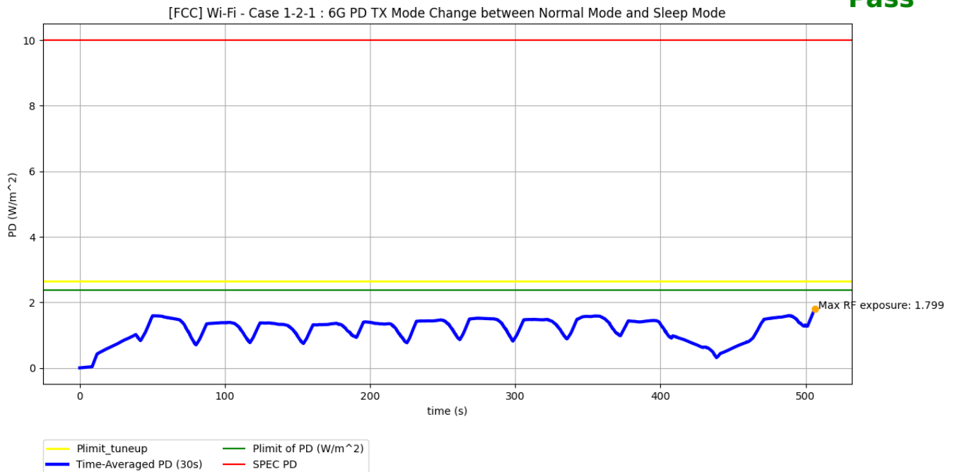
Figure 10-1 Time-averaged PD measurement for scenario 1-2-1
