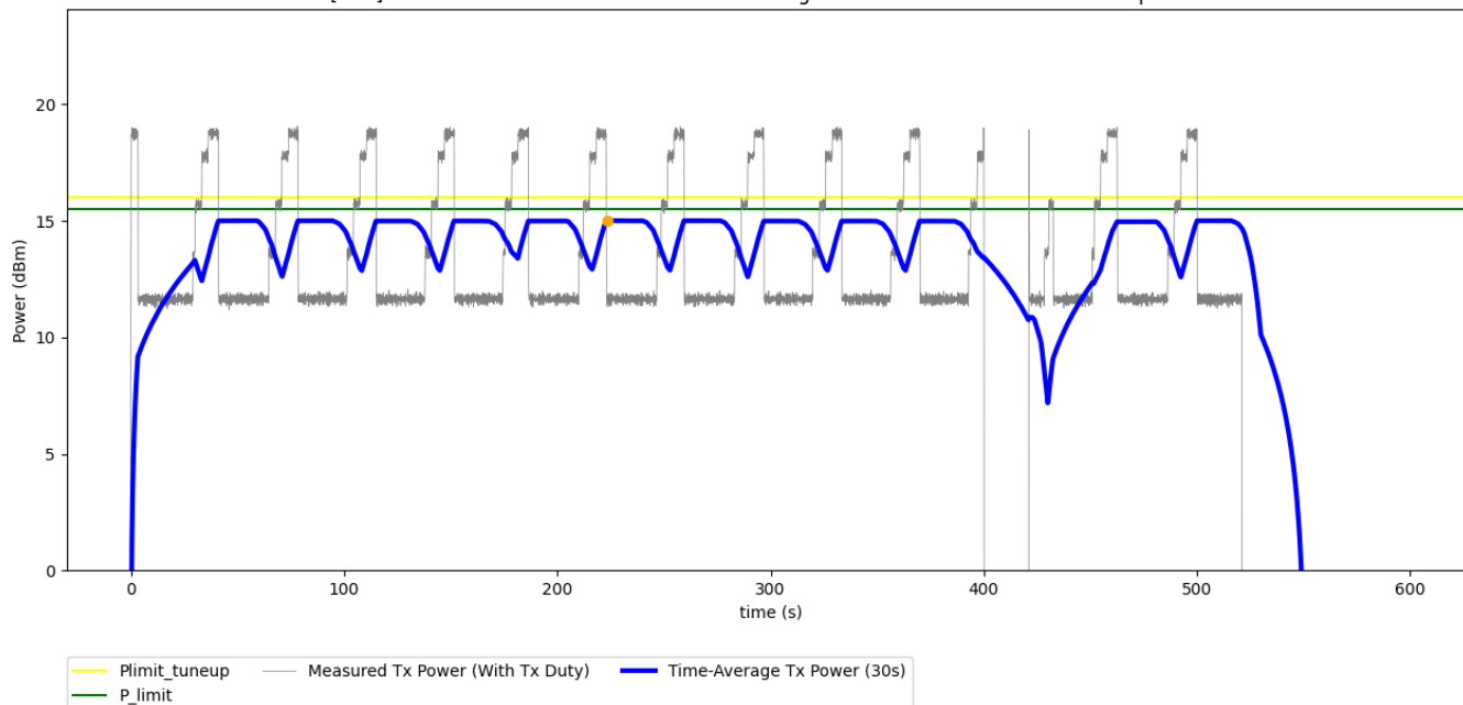
Figure 7-2 Time-averaged conducted TX power over time for test scenario 1-2-2
