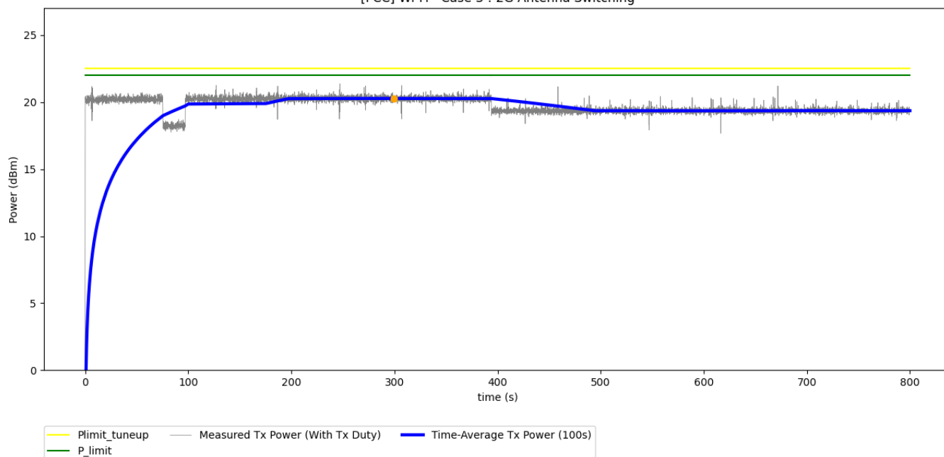
Figure 7-5 Time-averaged conducted TX power over time for test scenario 3
