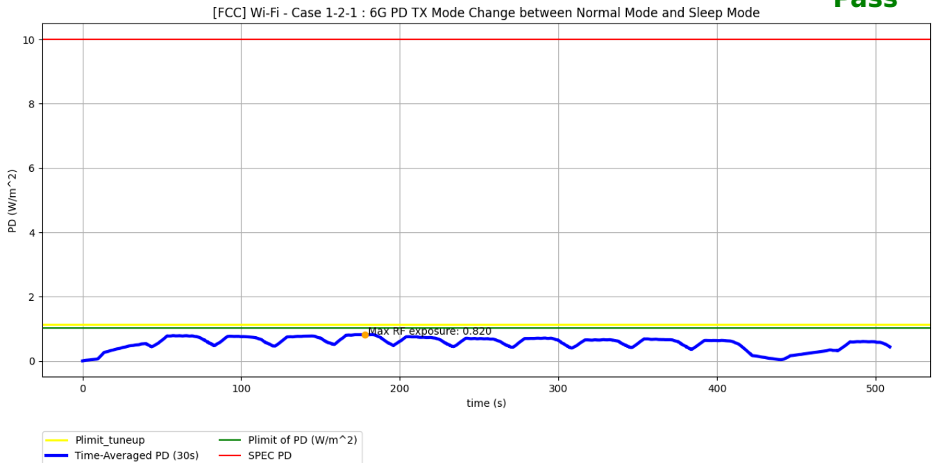
Figure 10-1 Time-averaged PD measurement for scenario 1-2-1
