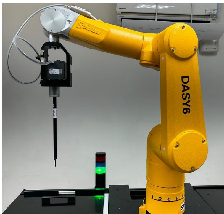
Fig.2 Photograph of the SAR measurement system
