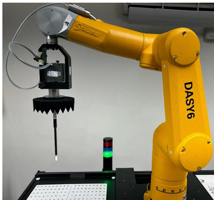
Fig.3 Photograph of the mmW measurement system
